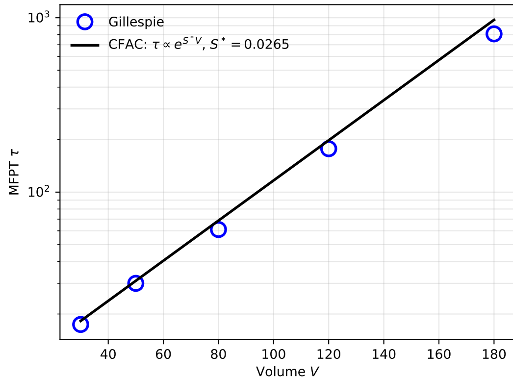
MFPT scales exponentially in V
