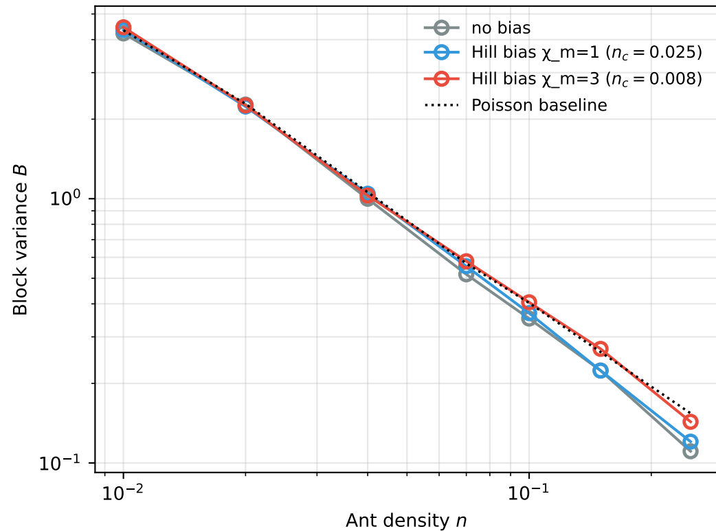
Block variance: bias increases clustering
