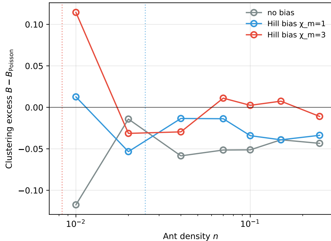
Clustering vs CFAC-KS prediction n_c
