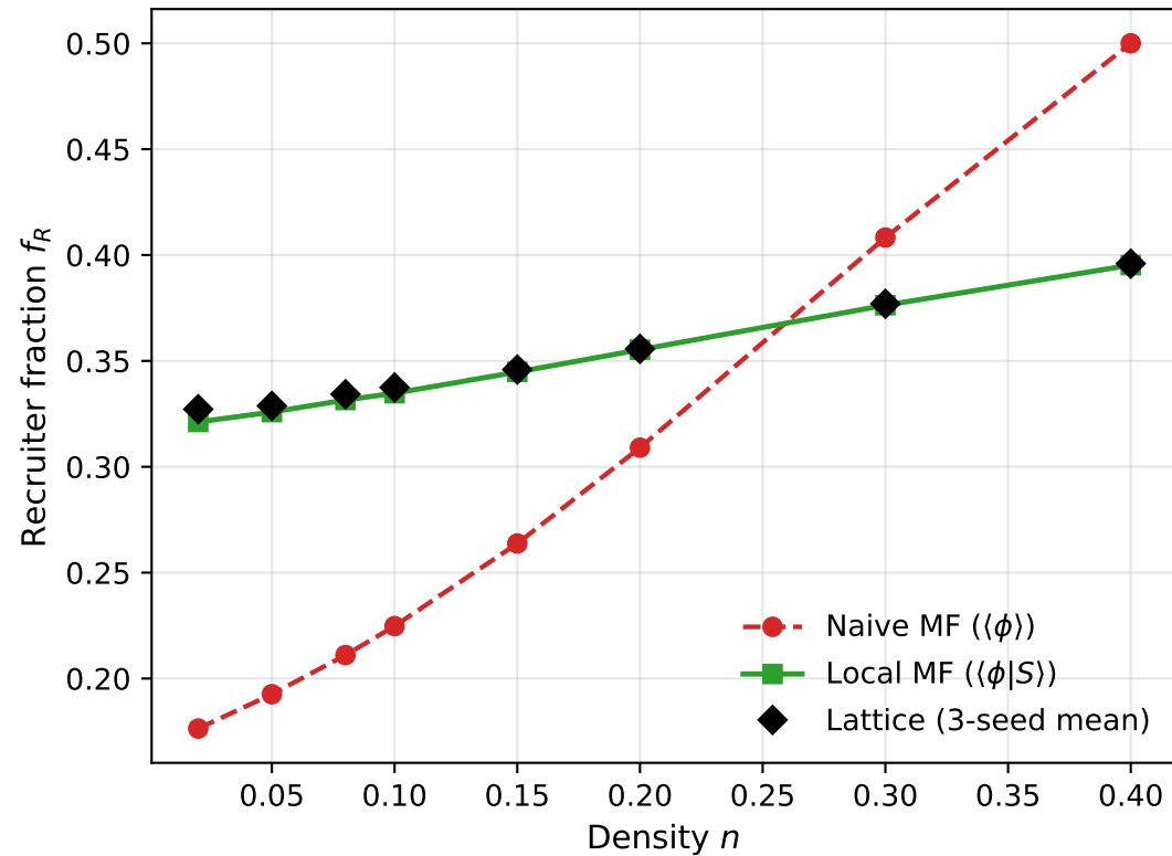
Tree-level MF vs lattice: canonical ant
