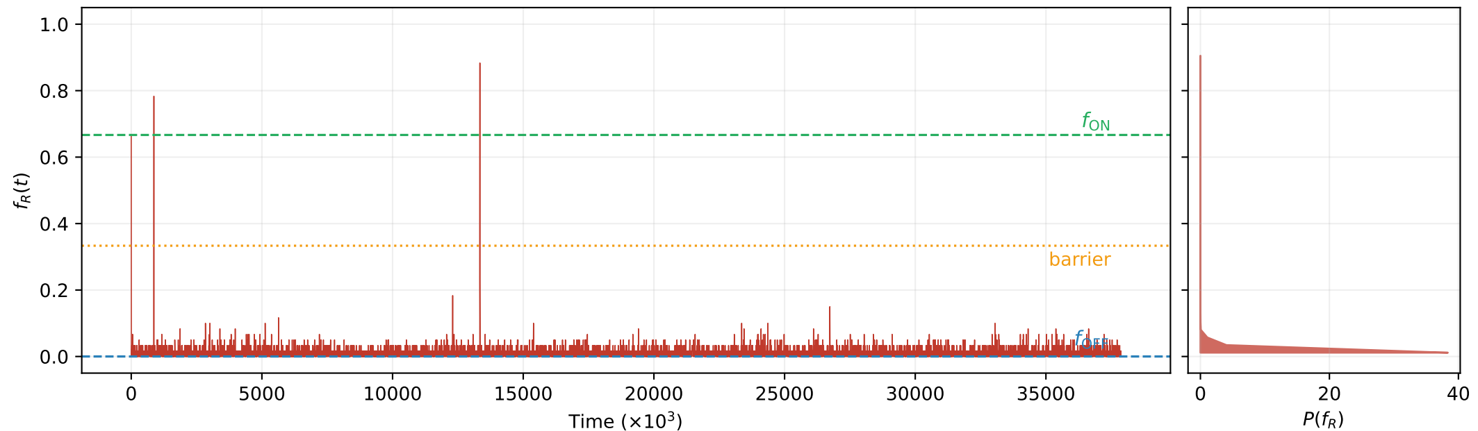
Colony state over \sim 37871 k time units: 109 ON \leftrightarrow OFF switches, typical dwell \sim 347 k units
