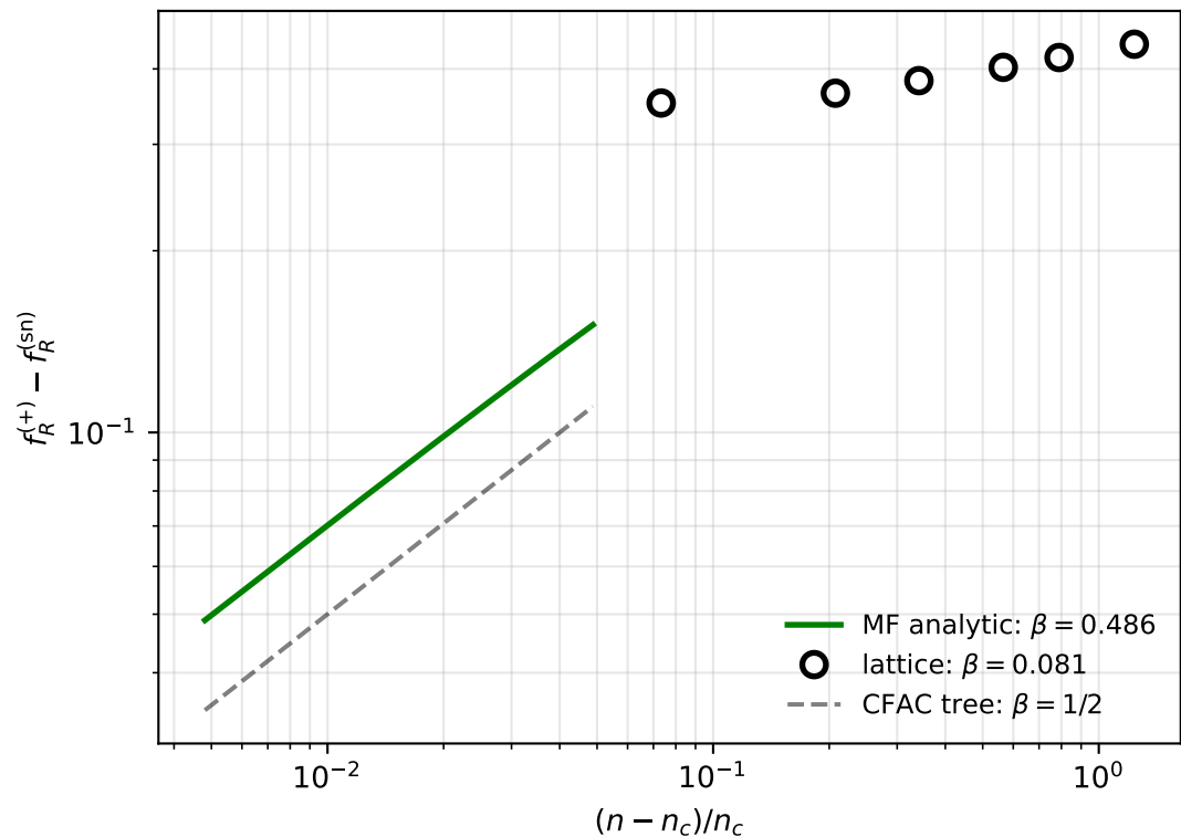
Order parameter exponent \beta at saddle-node
