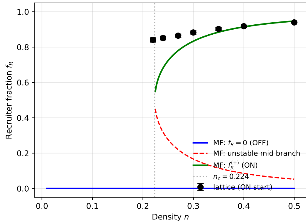
Cooperative canonical ant: saddle-node bifurcation
