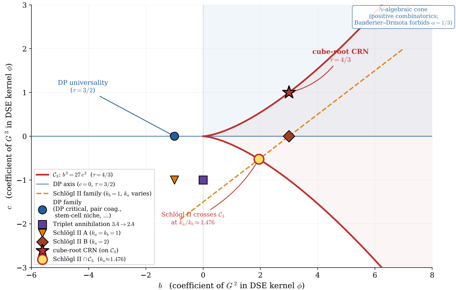
CRN universality classes as positions in DSE rate space (cubic slice; linear coefficient a suppressed, \mathcal{C}_3 is a -independent)
