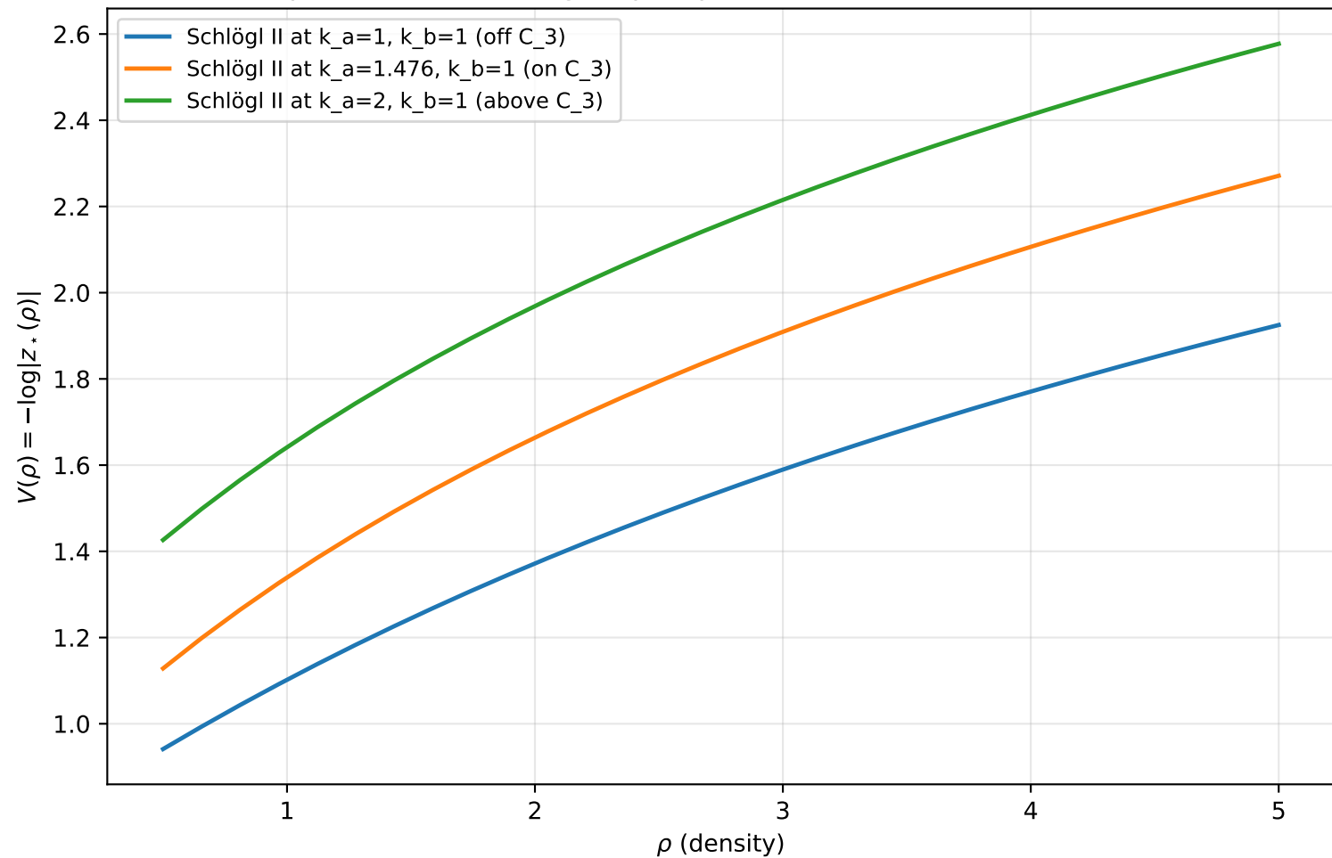
Experiment 12: Schlögl II quasipotential from CFAC branch radius
