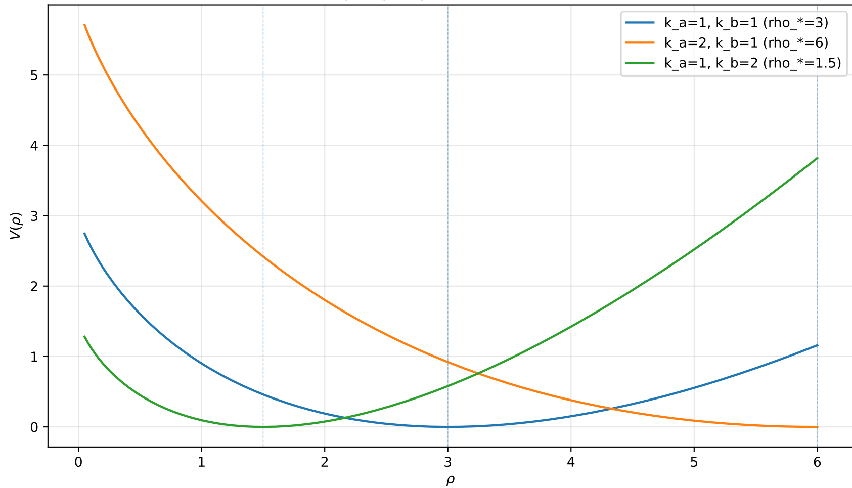
Schlögl II quasipotential (closed form)
