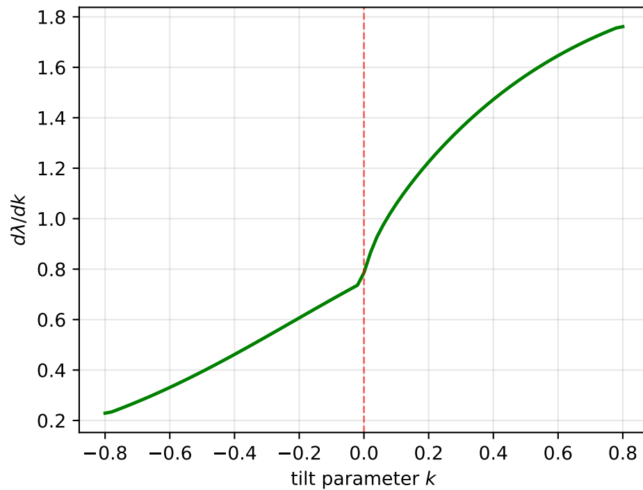
First derivative (mean current)
