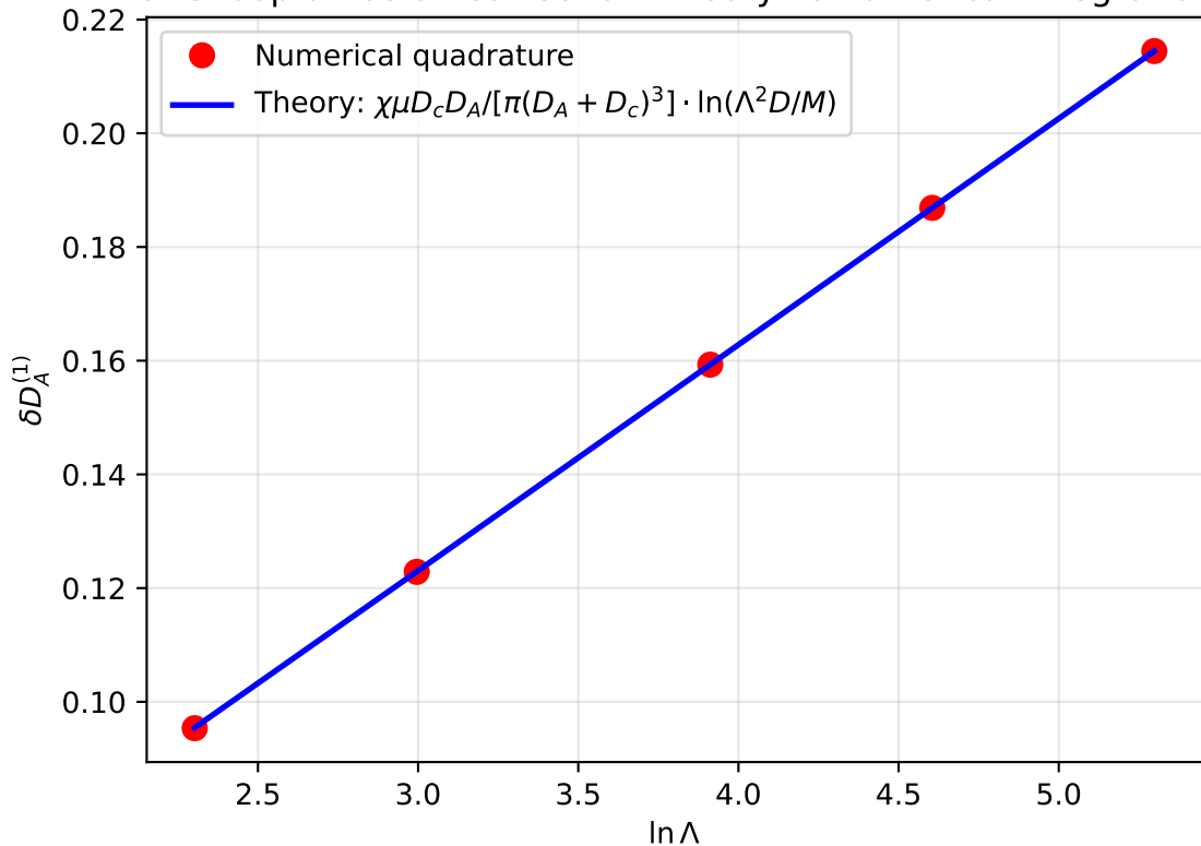
One-loop diffusion correction: theory vs numerical integration
