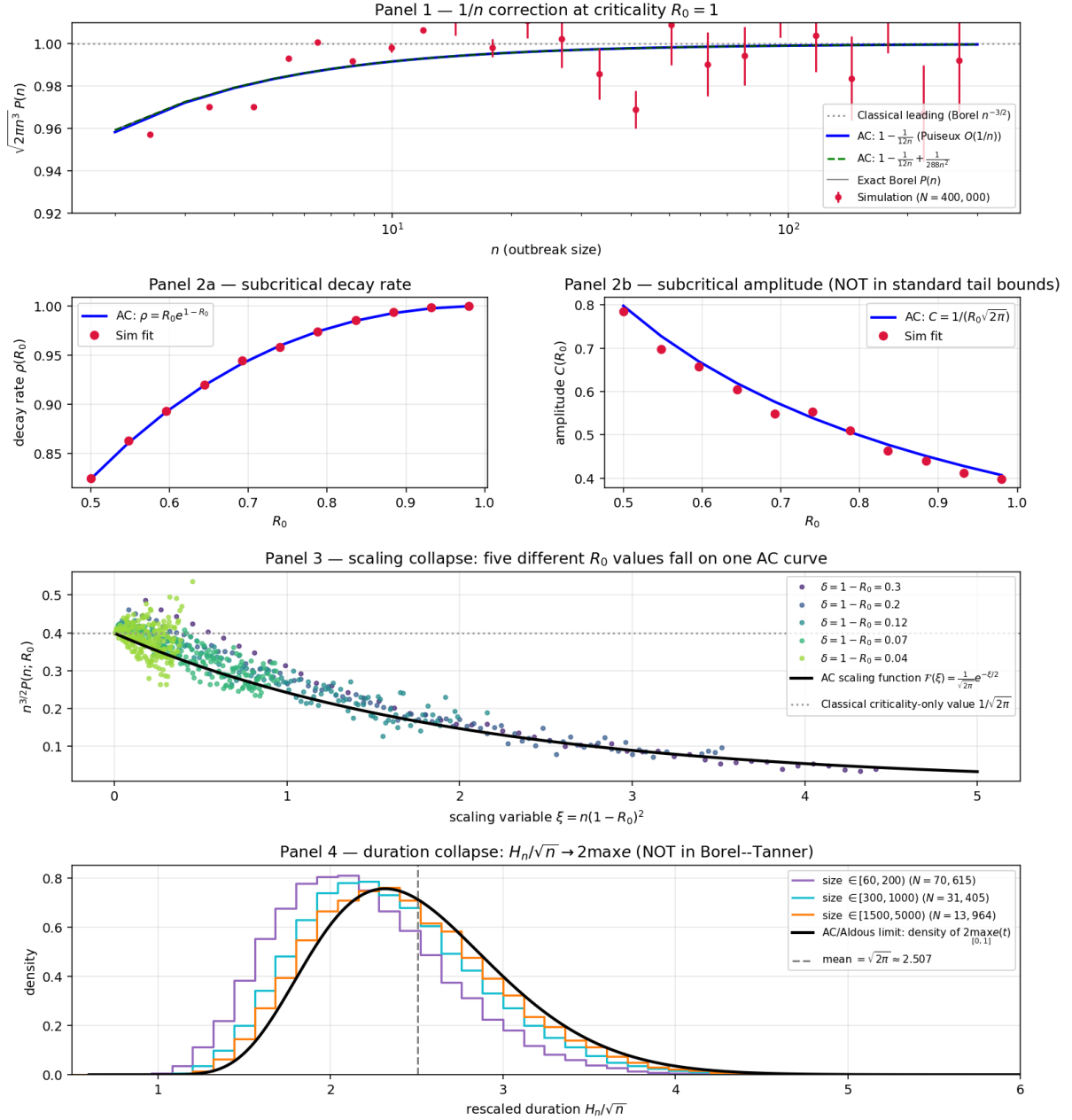
Figure 4: Three calibration panels (1–3) and one genuine-AC panel (4). Panel 1: rescaled PMF \sqrt{2\pi n^3} P(n) at R_0 = 1 ; the dip below 1 is the -1/(12n) correction, continued by +1/(288n^2) . Panel 2: subcritical decay \rho(R_0) = R_0 e^{1-R_0} and amplitude C(R_0) = 1/(R_0 \sqrt{2\pi}) . Panel 3: plotting n^{3/2} P(n; R_0) against \xi = n(1 - R_0)^2 collapses five values of R_0 onto \mathcal{F}(\xi) = (2\pi)^{-1/2} e^{-\xi/2} . Panels 1–3 are also obtainable from Stirling on the Borel–Tanner closed form. Panel 4 is what AC adds: histograms of the rescaled outbreak duration H_n/\sqrt{n} at criticality, conditioned on three disjoint size bins ( n \in [60, 200) , [300, 1000) , [1500, 5000) ). All three histograms collapse onto the single Aldous limit law (black curve) — the density of 2 \max_{[0,1]} e(t) , where e is the normalised Brownian excursion — with sample mean \sqrt{2\pi} \approx 2.507 . Panel 4 is silent in Borel–Tanner: the closed-form pmf knows total size, not duration. Reproduced by simulations/sir_ac_demo.py .
