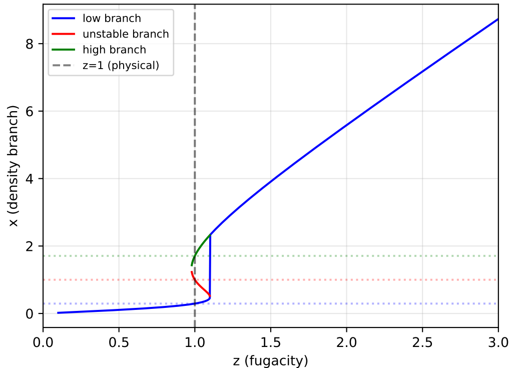
Schlögl: a=0.5 , \lambda=3.0 , \delta=2.5 S_{\text{inst}} = 0.0391
