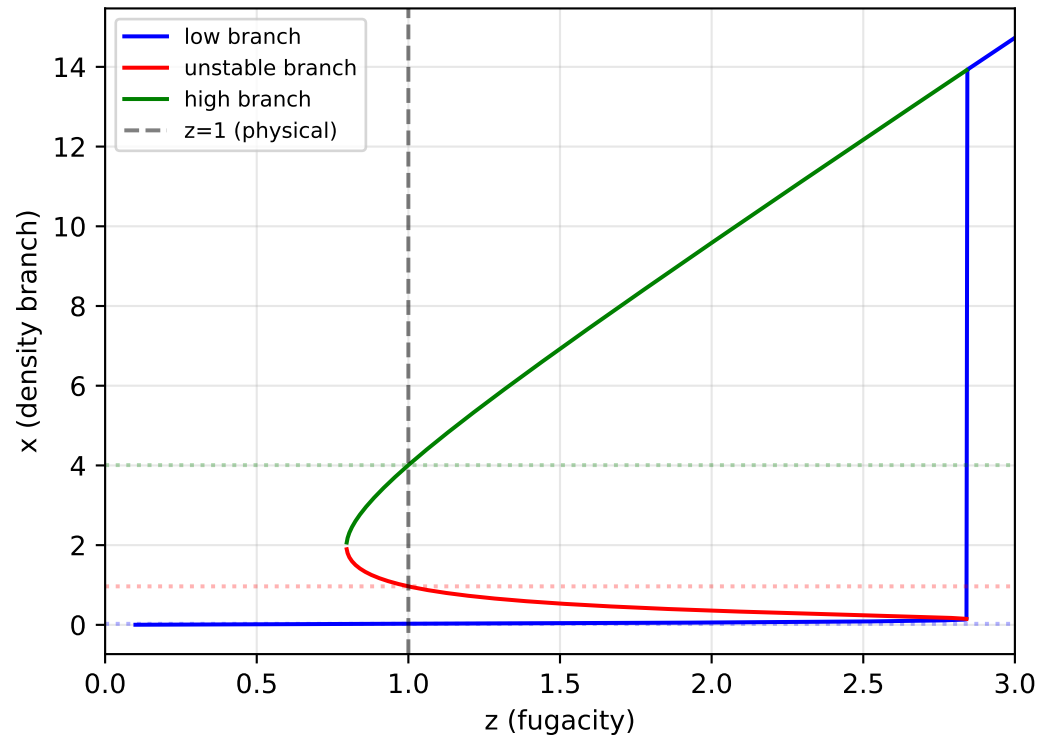
Strong coupling: a=0.1 , \lambda=5.0 , \delta=4.0 S_{\text{inst}} = 0.4558
