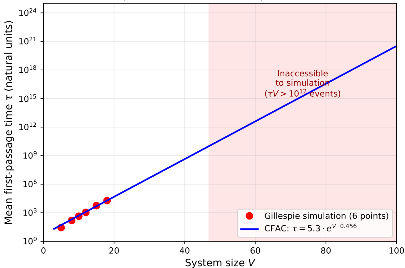
CFAC extrapolates nucleation rates beyond simulation reach
