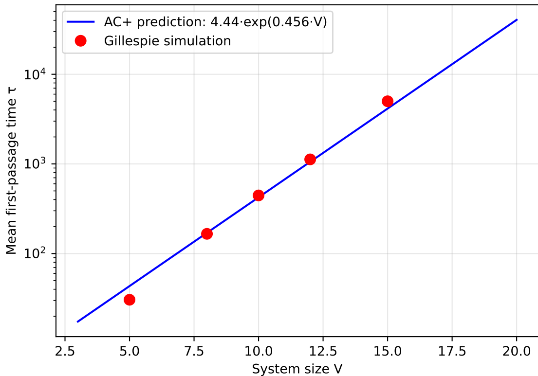
Nucleation rate from AC+ vs simulation
