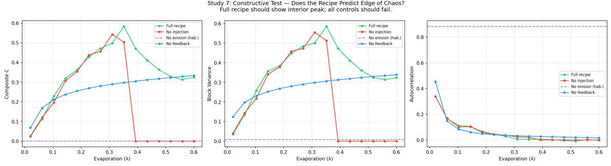
Figure 24: Constructive test of the three-ingredient recipe. Green: full recipe (interior peak at \lambda = 0.35 , confirming edge of chaos). Red: coupled deposition (tracks full recipe until absorbing state kills it at \lambda \geq 0.39 ). Purple dashed: habituation with no decay (frozen, C \approx 0 ). Blue: no positive feedback (monotonic rise, no peak). Three of four predictions confirmed; the fourth reveals a refinement about the absorbing state.
