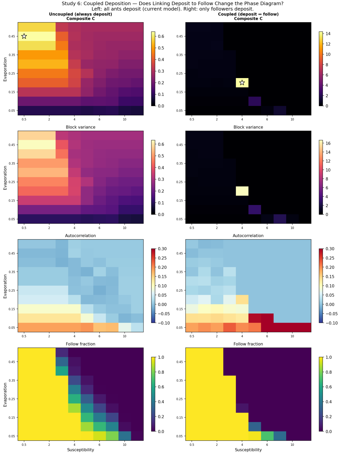
Figure 23: Coupled (right) vs uncoupled (left) deposition. The coupled model shows a sharp alive/dead boundary (bottom row). Extreme block variance at the boundary reflects dying clusters, not edge of chaos.
