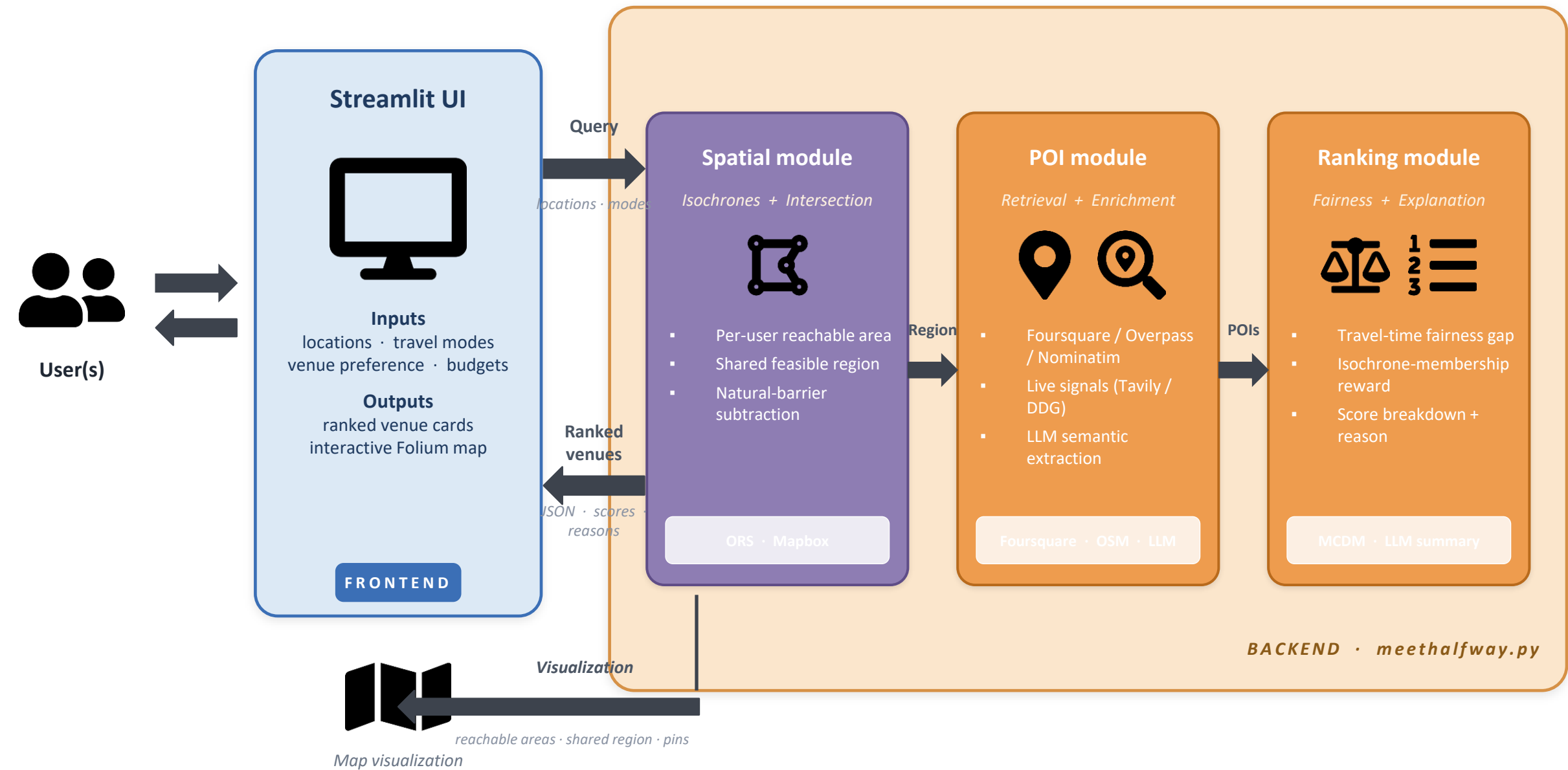
Figure: The MeetHalfway system architecture
