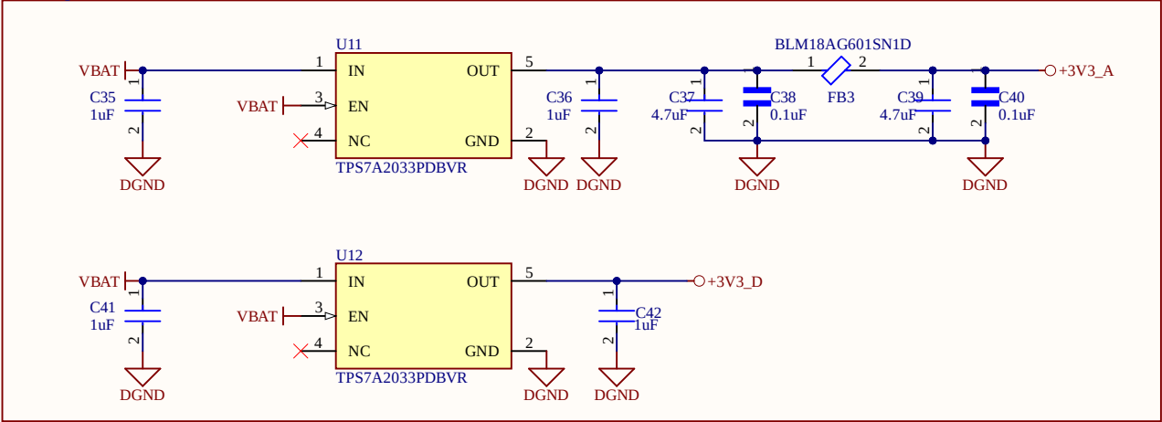
Power Regulation
