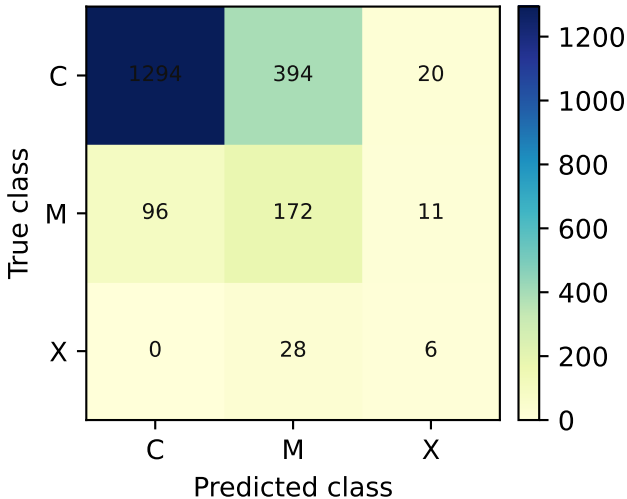
Test confusion matrix
