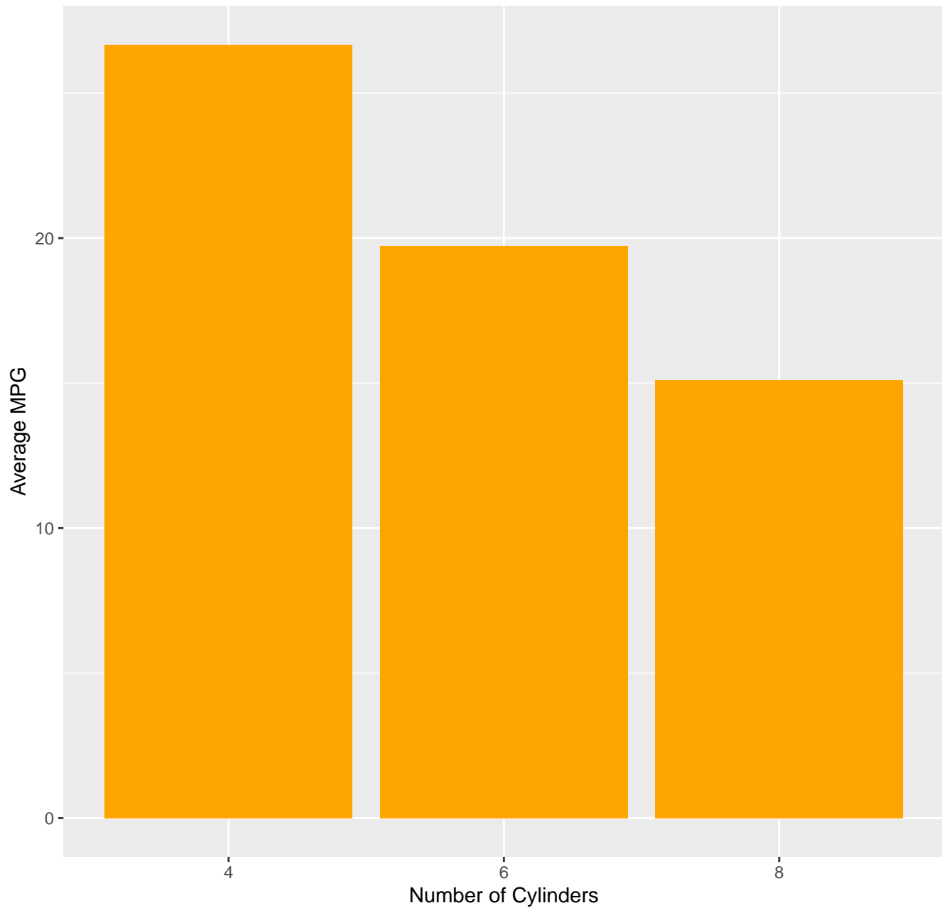
Average MPG by Number of Cylinders
