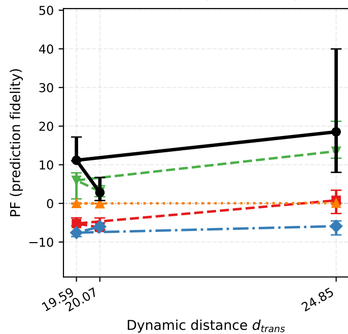
MiniGrid (Discrete)
