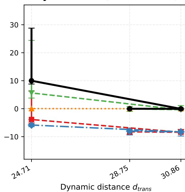
Gymnasium (Continuous)
