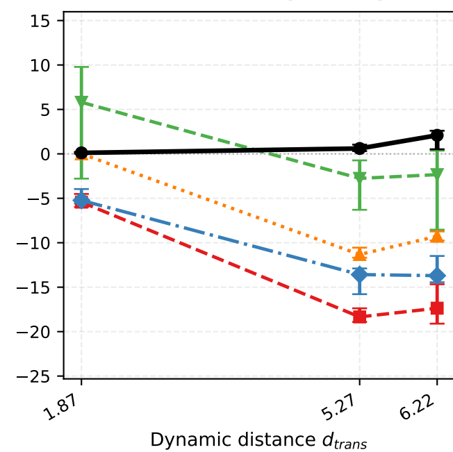
DMControl (Visual)
