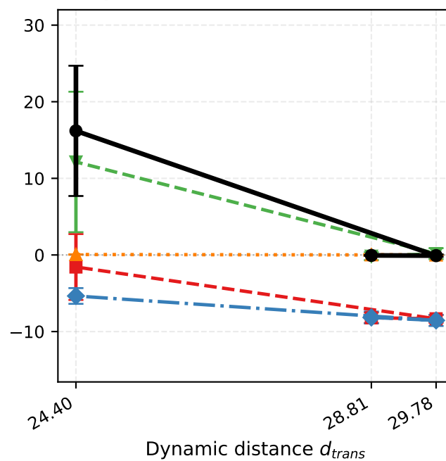
Gymnasium (Continuous)
