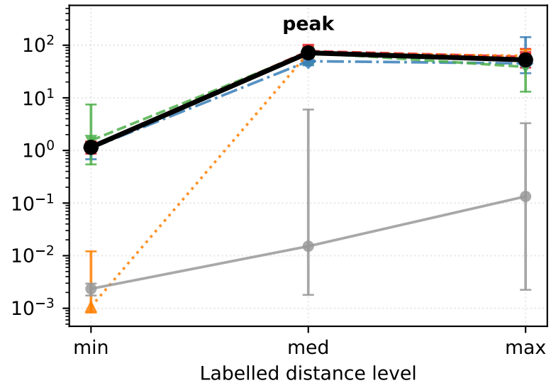
DMControl (visual)
