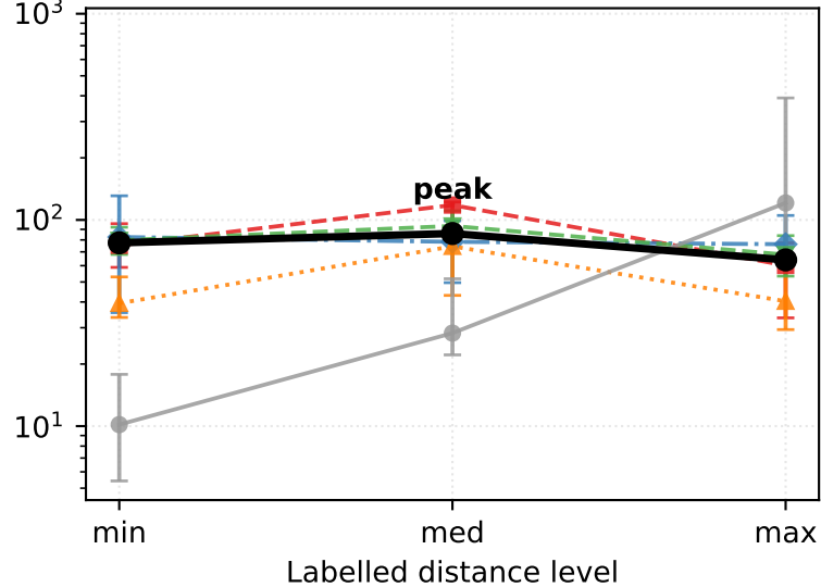
Gymnasium (continuous)
