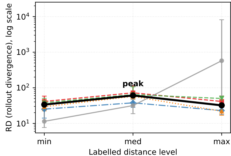
MiniGrid (discrete)
