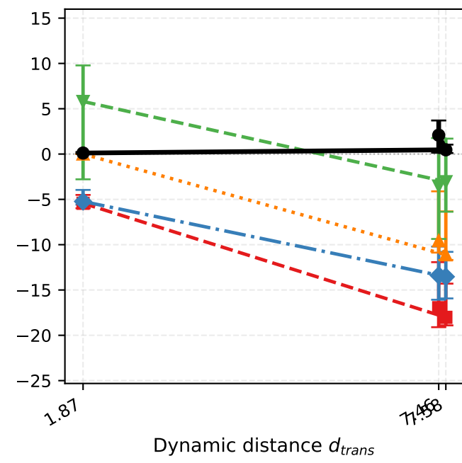
DMControl (Visual)
