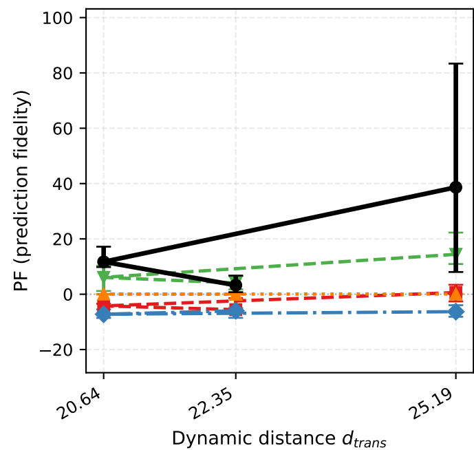
MiniGrid (Discrete)
