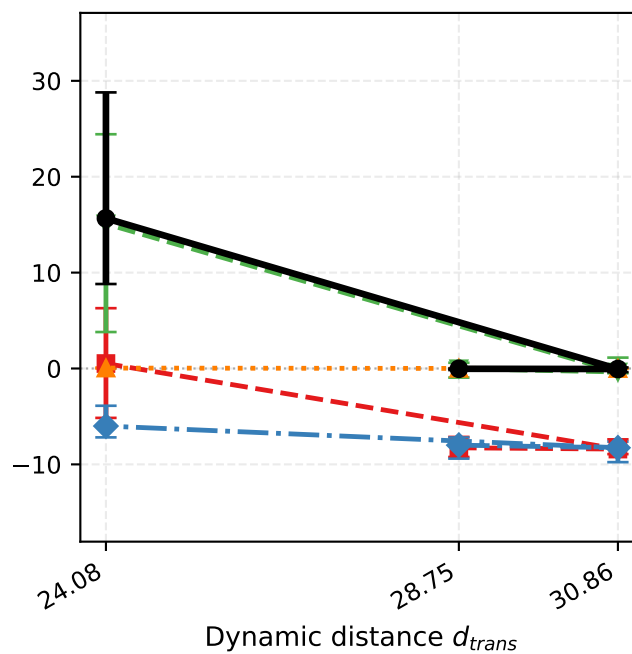
Gymnasium (Continuous)
