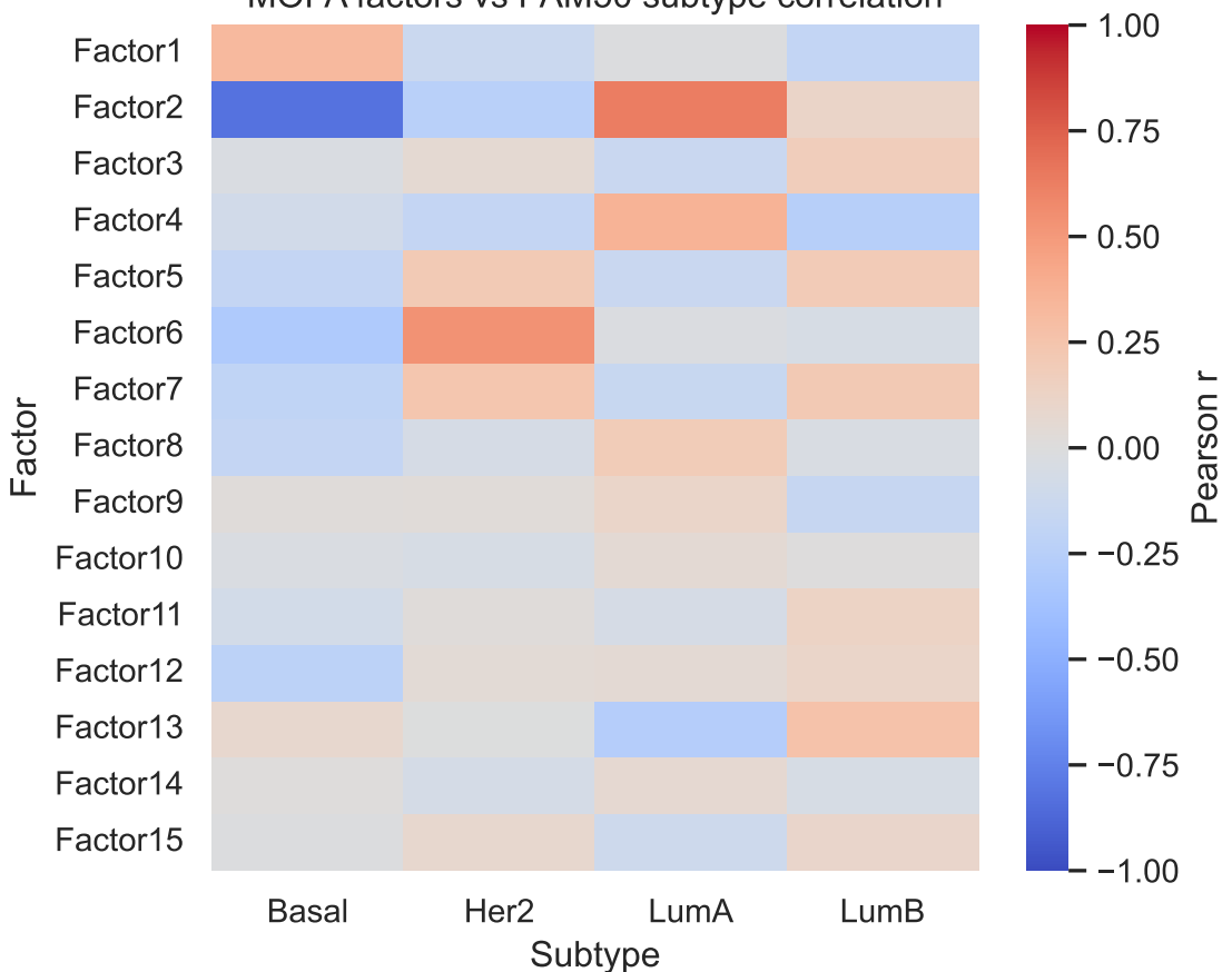
MOFA factors vs PAM50 subtype correlation
