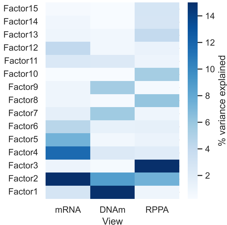
MOFA - R 2 per factor and view
