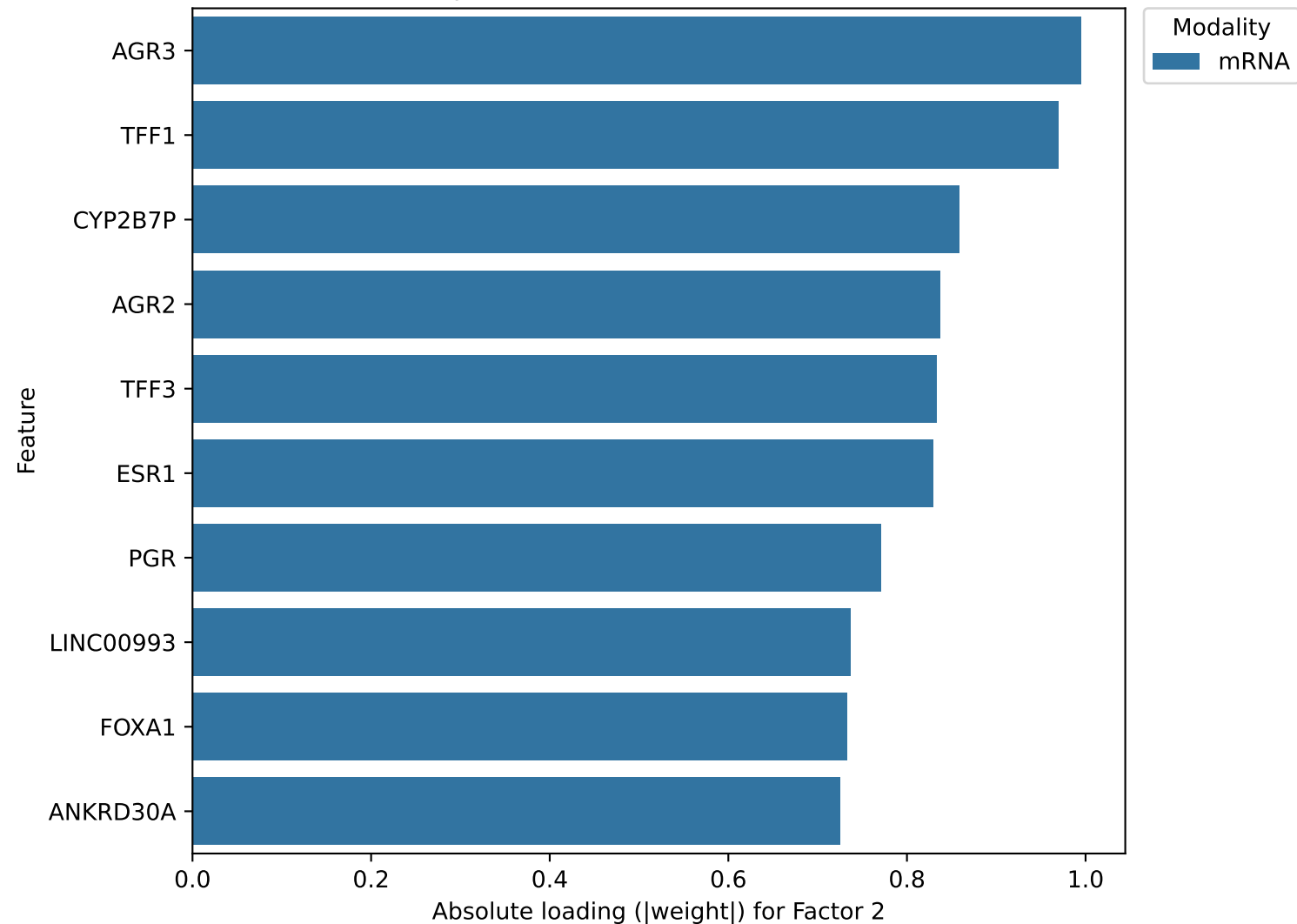
Top 10 MOFA features for Factor 2
