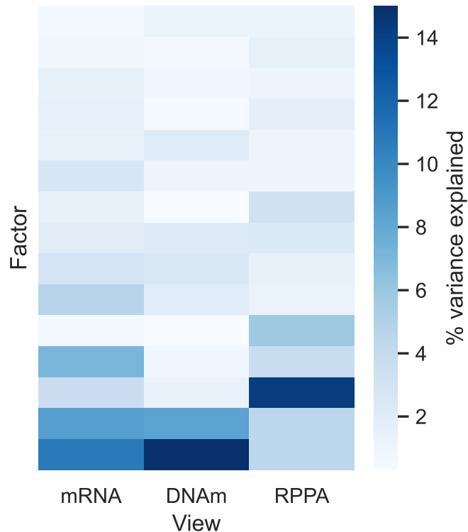
Combined_PCA - R 2 per factor and view
