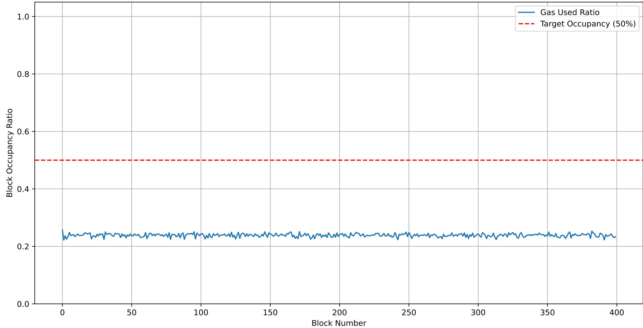
Block Occupancy Ratio (Max Gas: 150M) - low_demand
