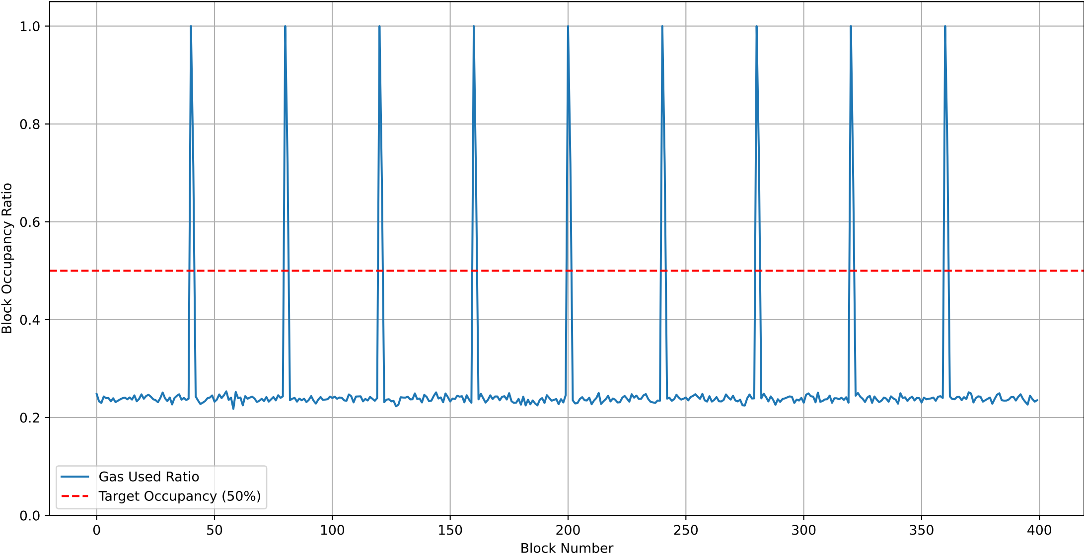
Block Occupancy Ratio (Max Gas: 150M) - spike_demand
