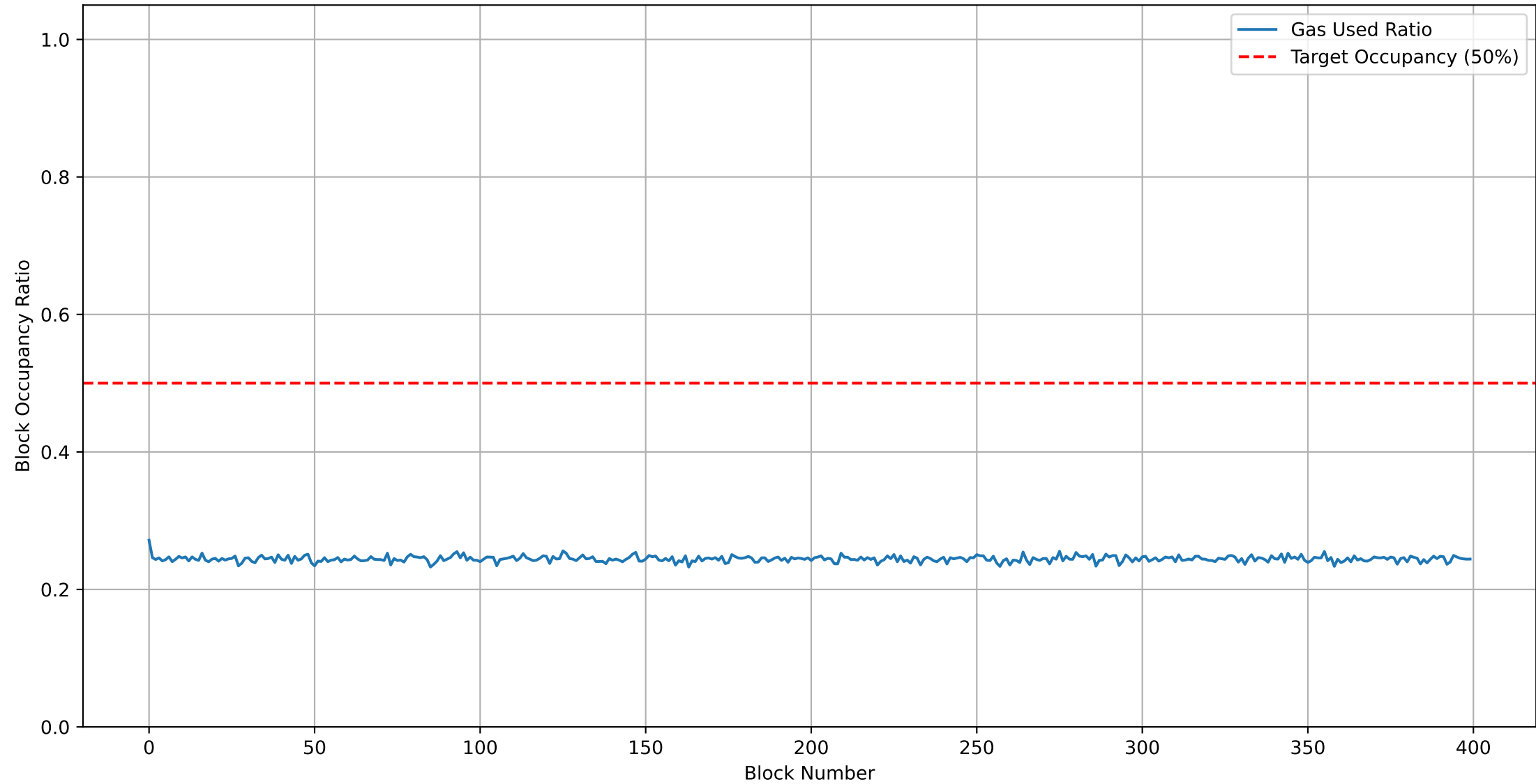
Block Occupancy Ratio (Max Gas: 300M) - low_demand
