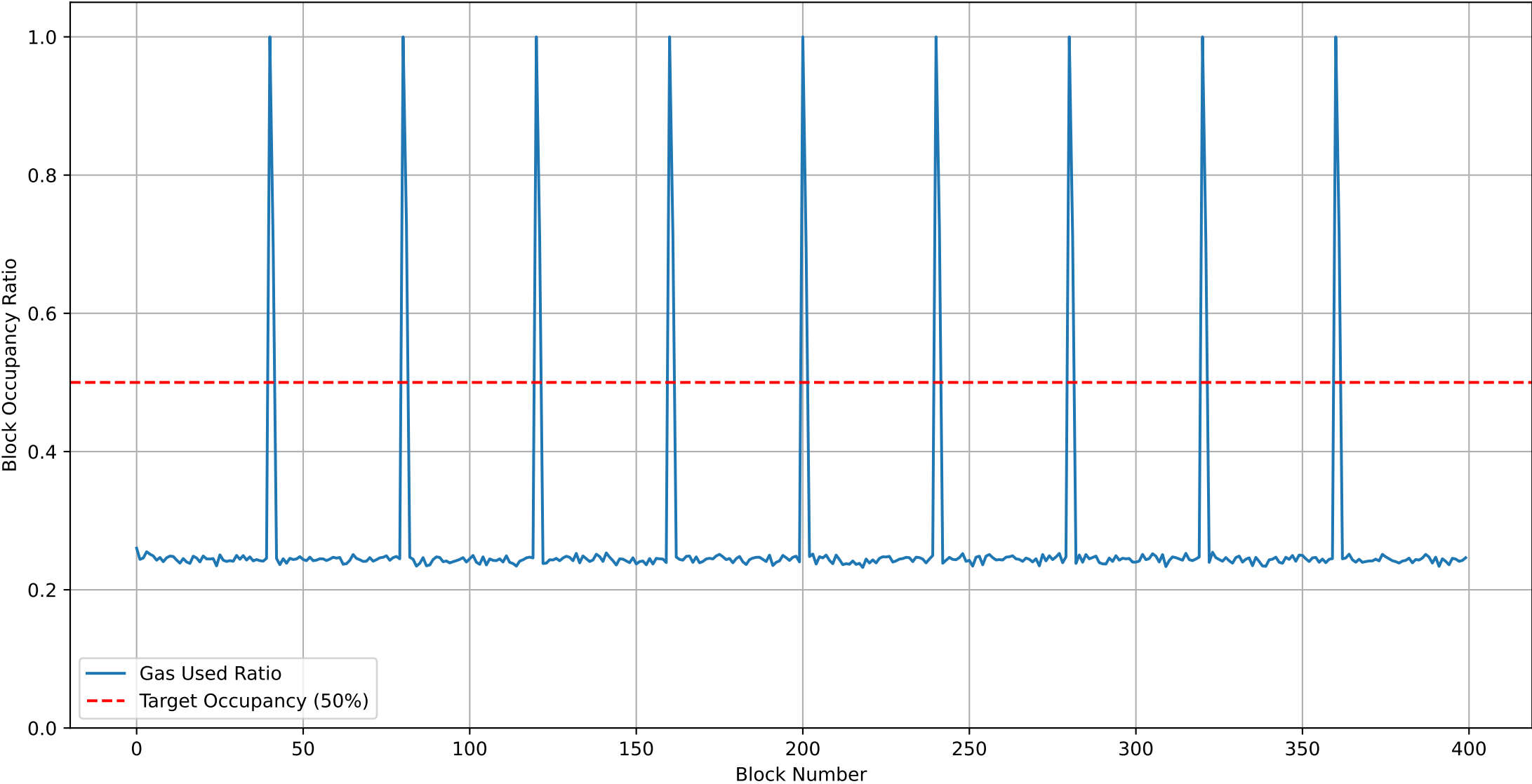
Block Occupancy Ratio (Max Gas: 300M) - spike_demand
