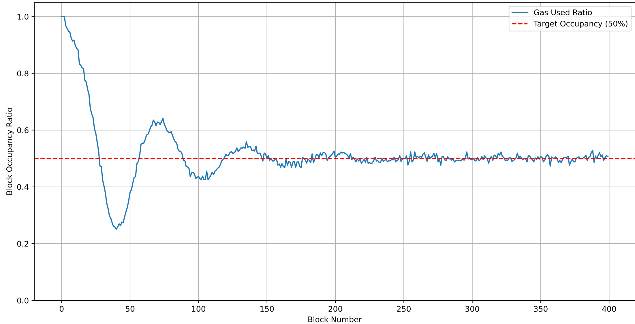
Block Occupancy Ratio (high_demand - 150M Max Gas)
