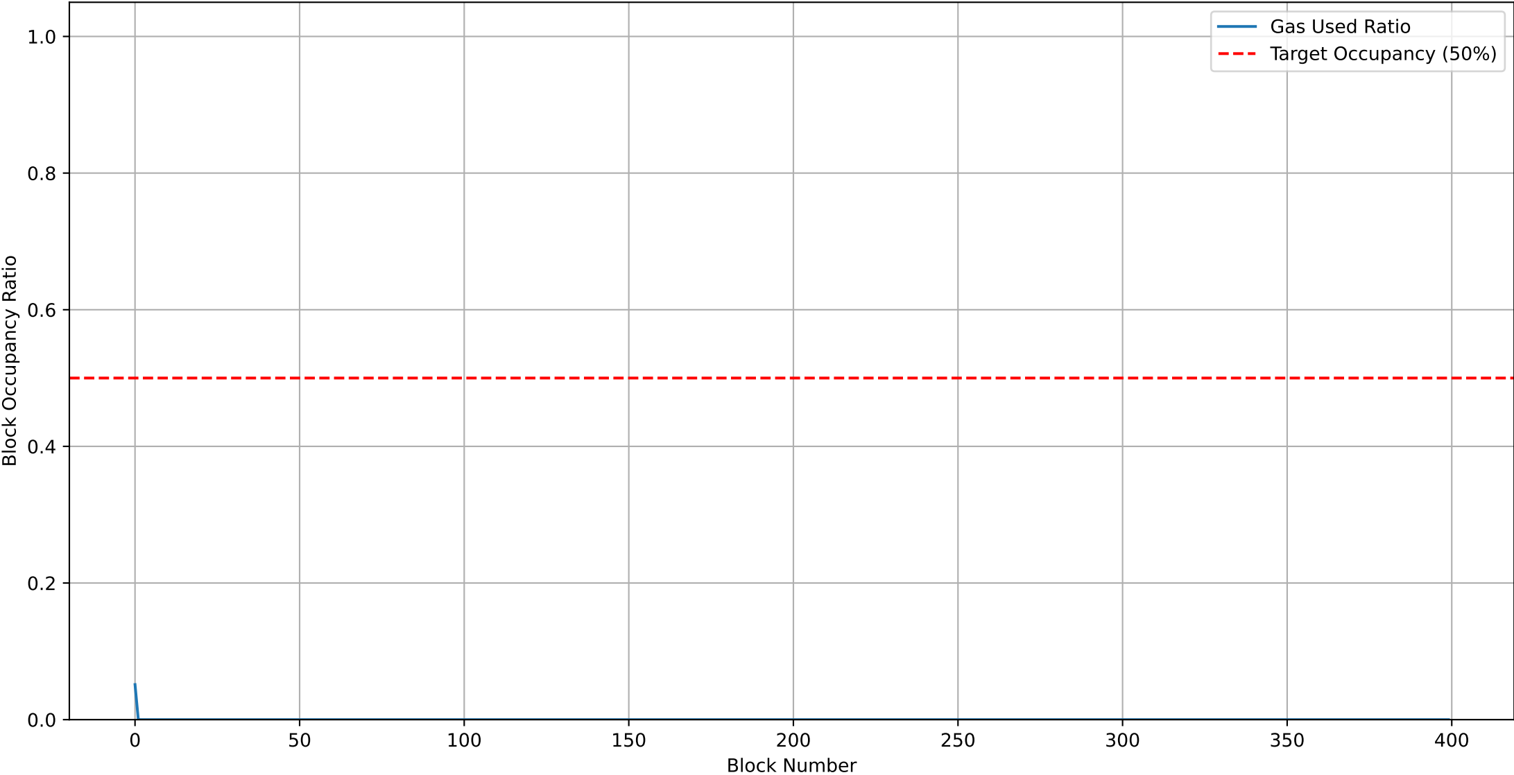
Block Occupancy Ratio (spam_demand - 150M Max Gas)
