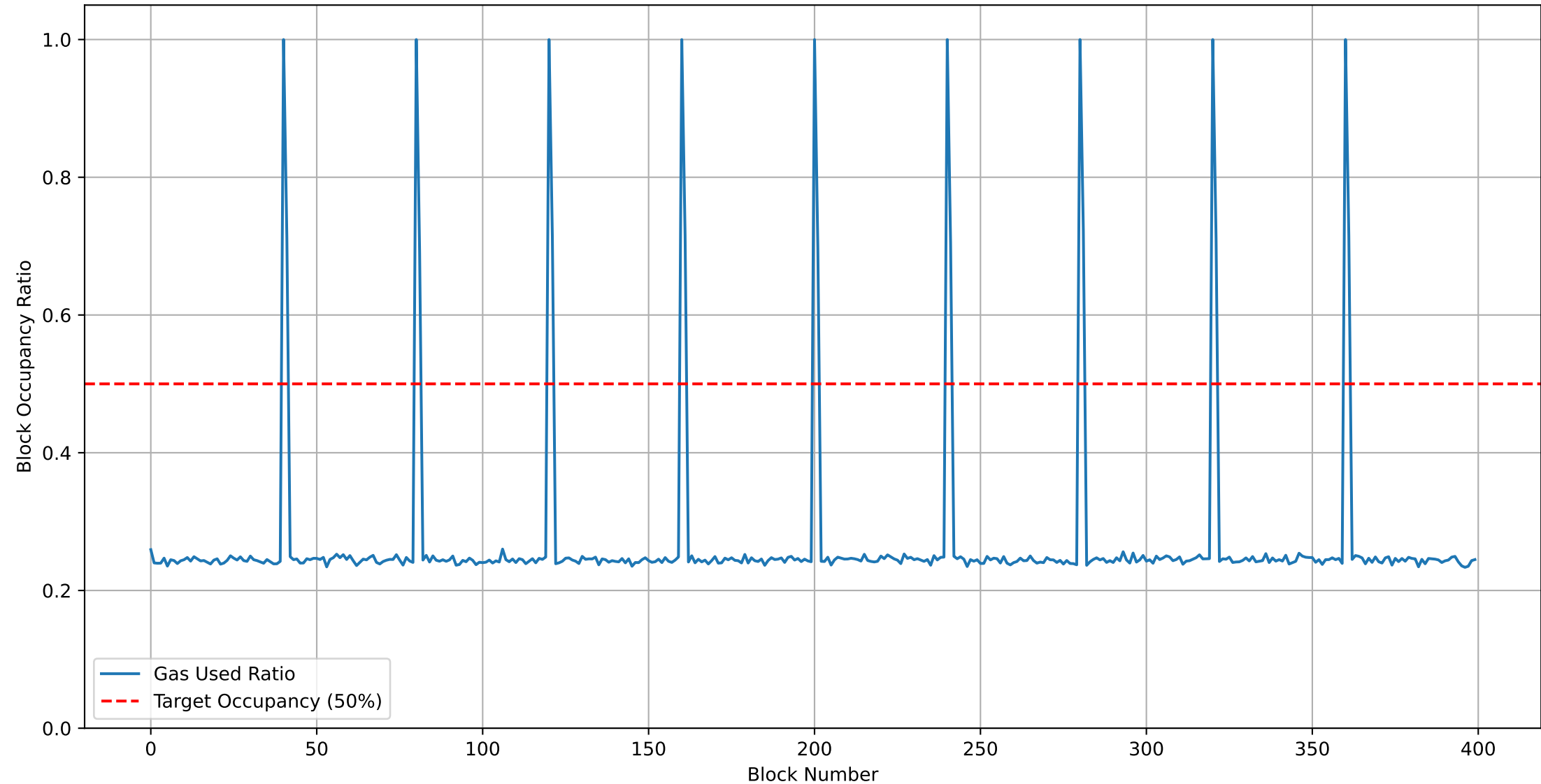
Block Occupancy Ratio (spike_demand - 300M Max Gas)
