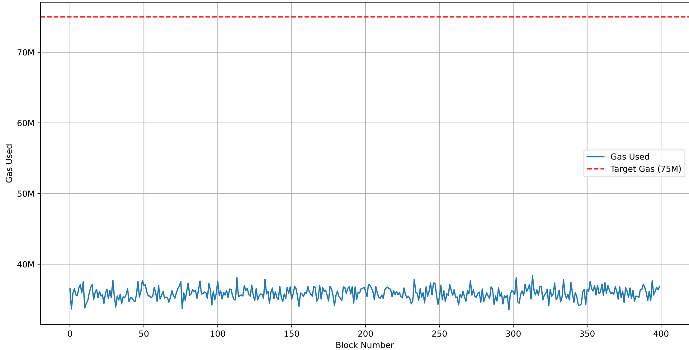
Gas Used vs. Target (Raw) (low_demand - 150M Max Gas)
