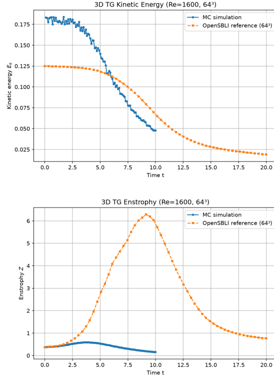
图 5: Phase 3 3D Taylor-Green 拟涡能随时间变化曲线 ( 64^3 网格, dt = 0.1 , T = 10s , \nu = 0.000625 )
