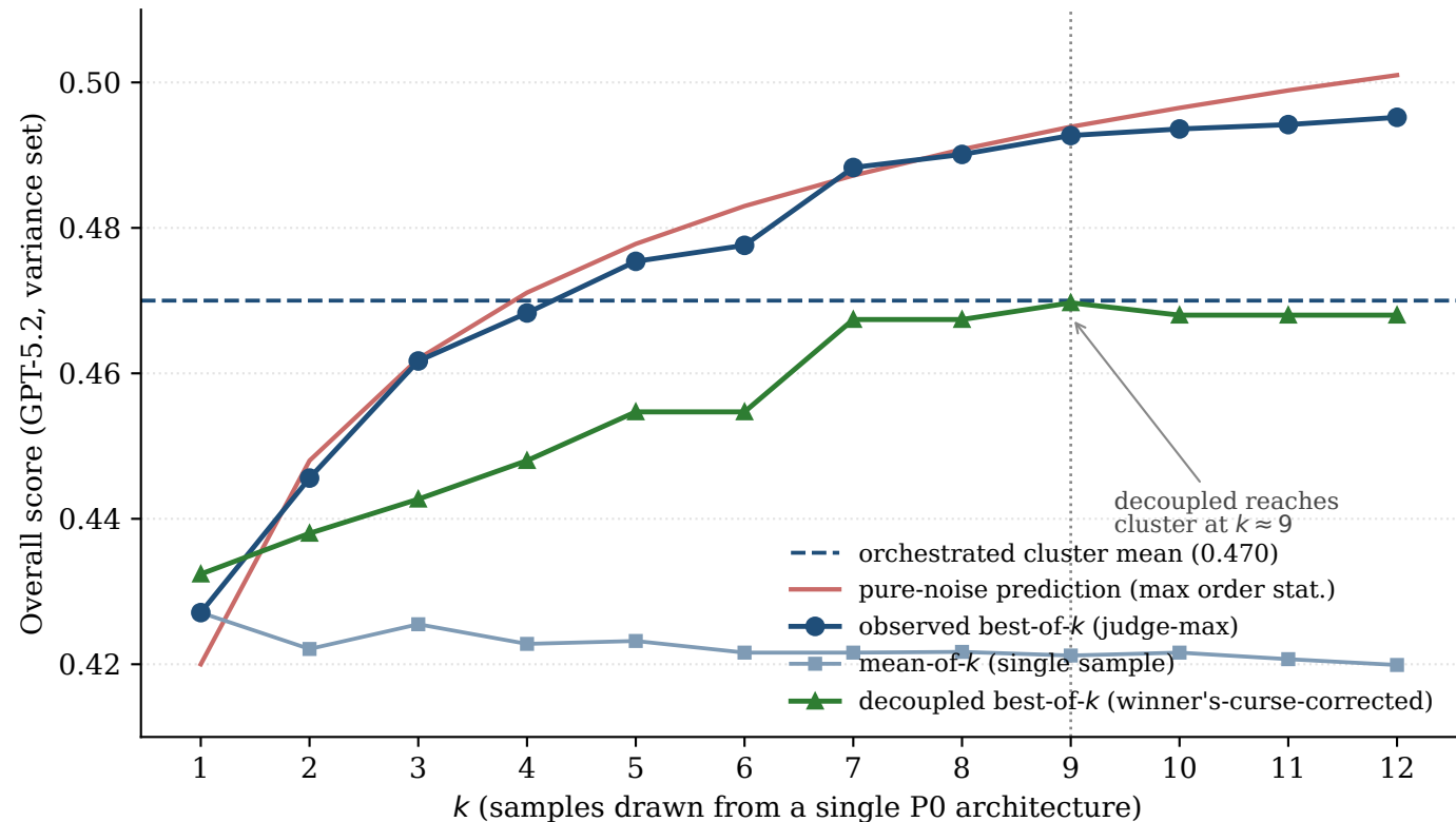
Best-of- k gains track judge-noise capitalisation, not quality
