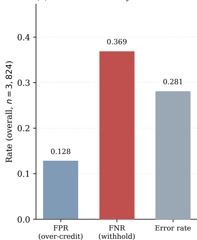
(b) Pooled error is asymmetric
