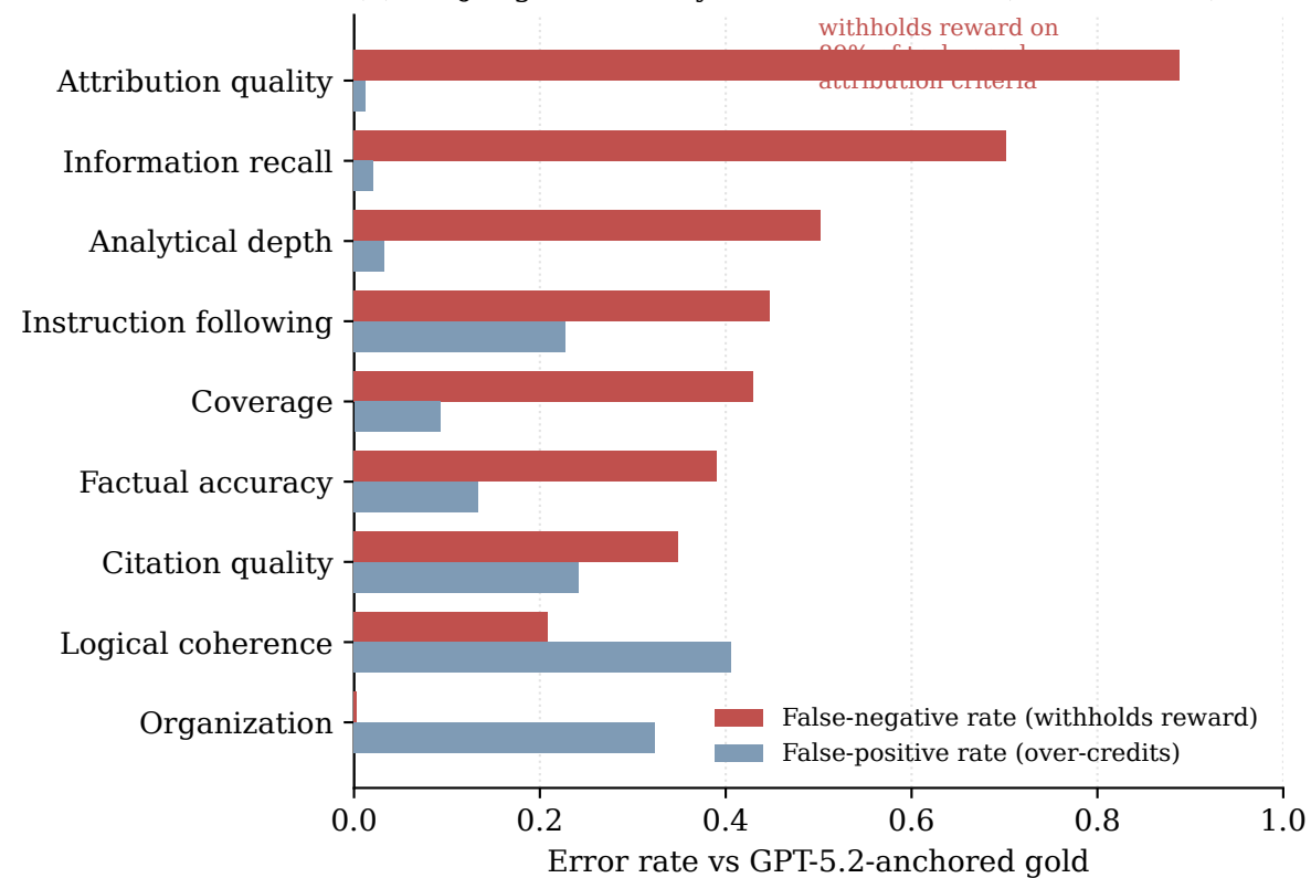
(a) DR-Judge-7B mostly withholds reward (FNR \gg FPR)
