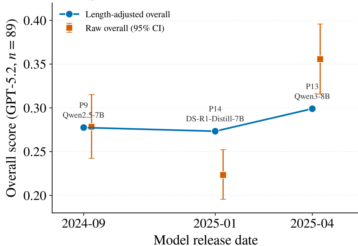
(a) Vintage-date axis, frozen GGUF scaffold ( \sim 7\text{--}8\text{B} )
