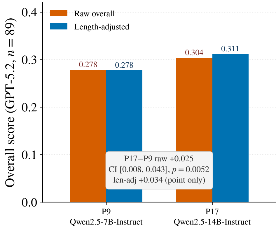
(b) Capacity axis at fixed 2024-09 vintage (7B \rightarrow 14B)
