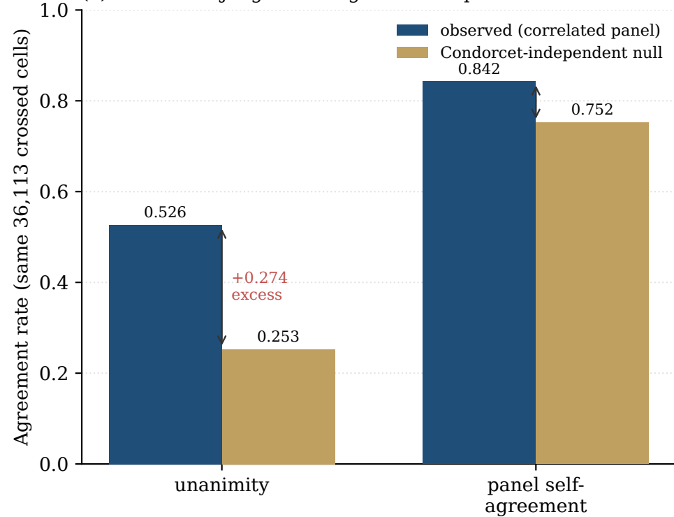
(a) Correlated judges over-agree vs independence
