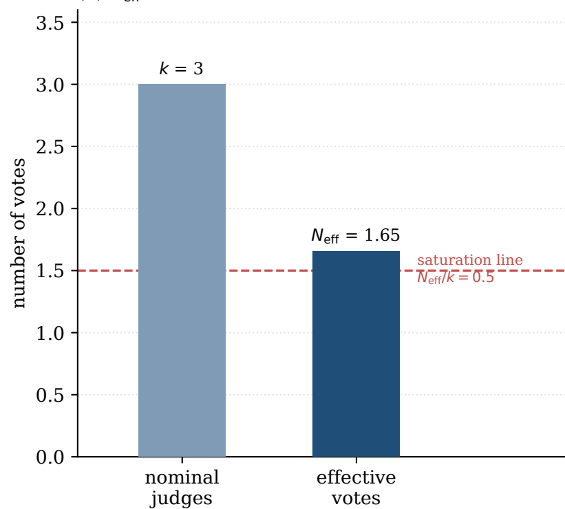
(b) N_{\text{eff}}/k = 0.552
