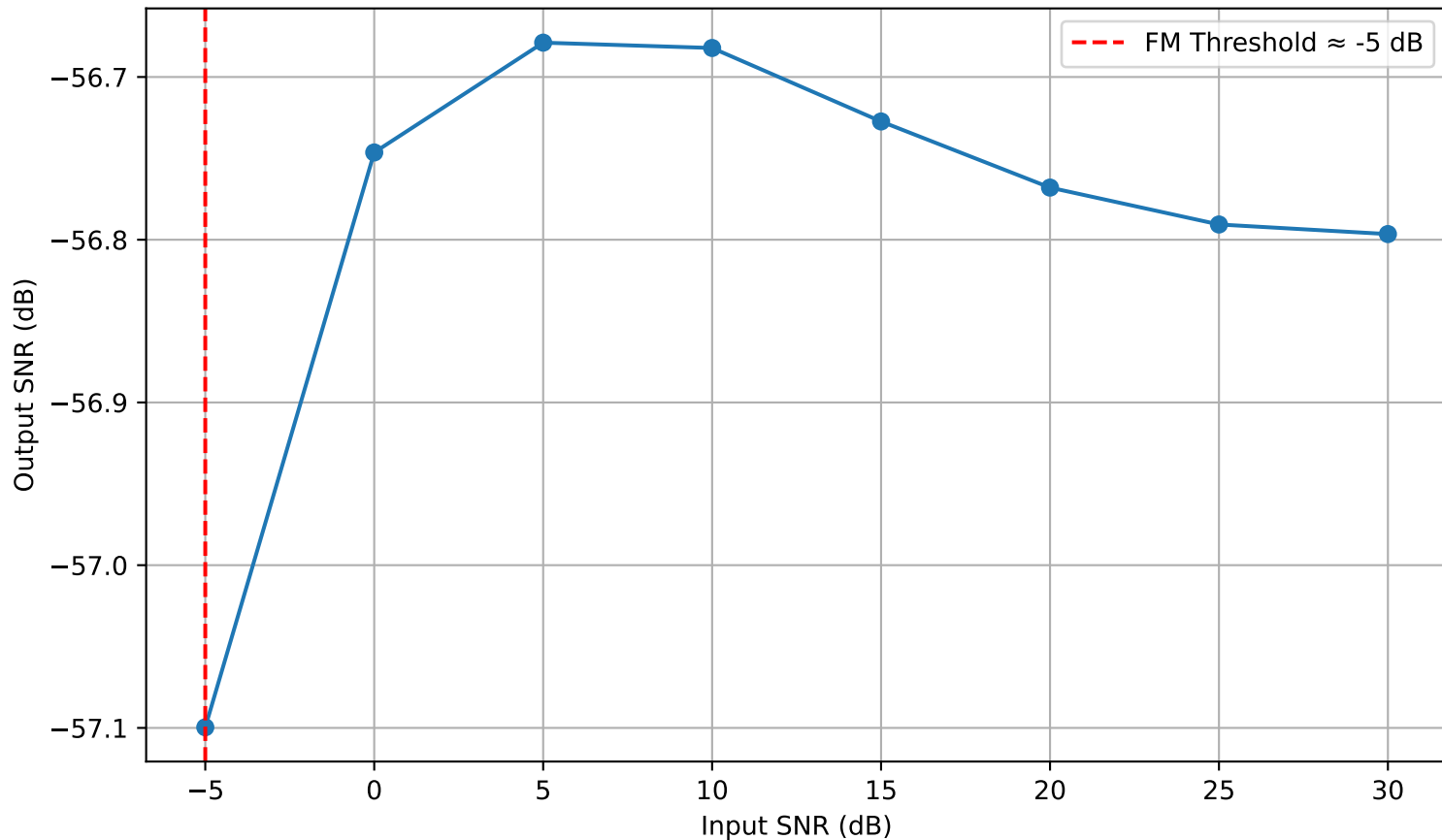
Output SNR vs Input SNR — WBFM SUPER
