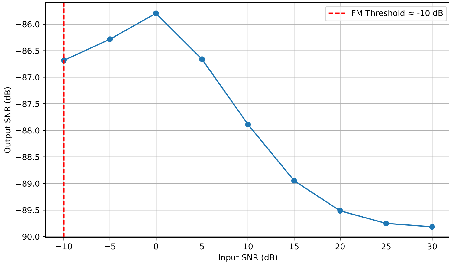
Output SNR vs Input SNR — WBFM TRF
