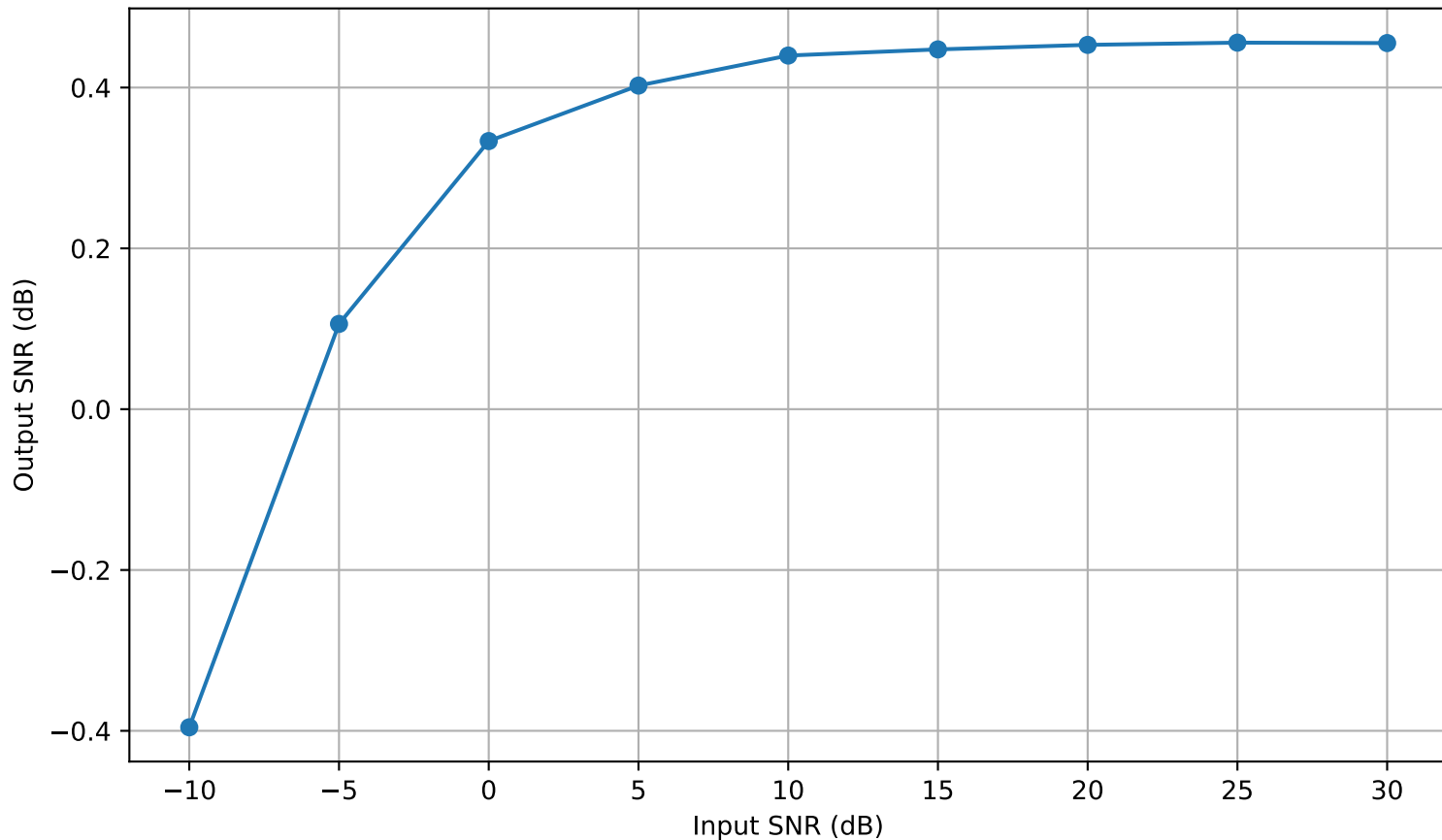
Output SNR vs Input SNR — AM SUPER
