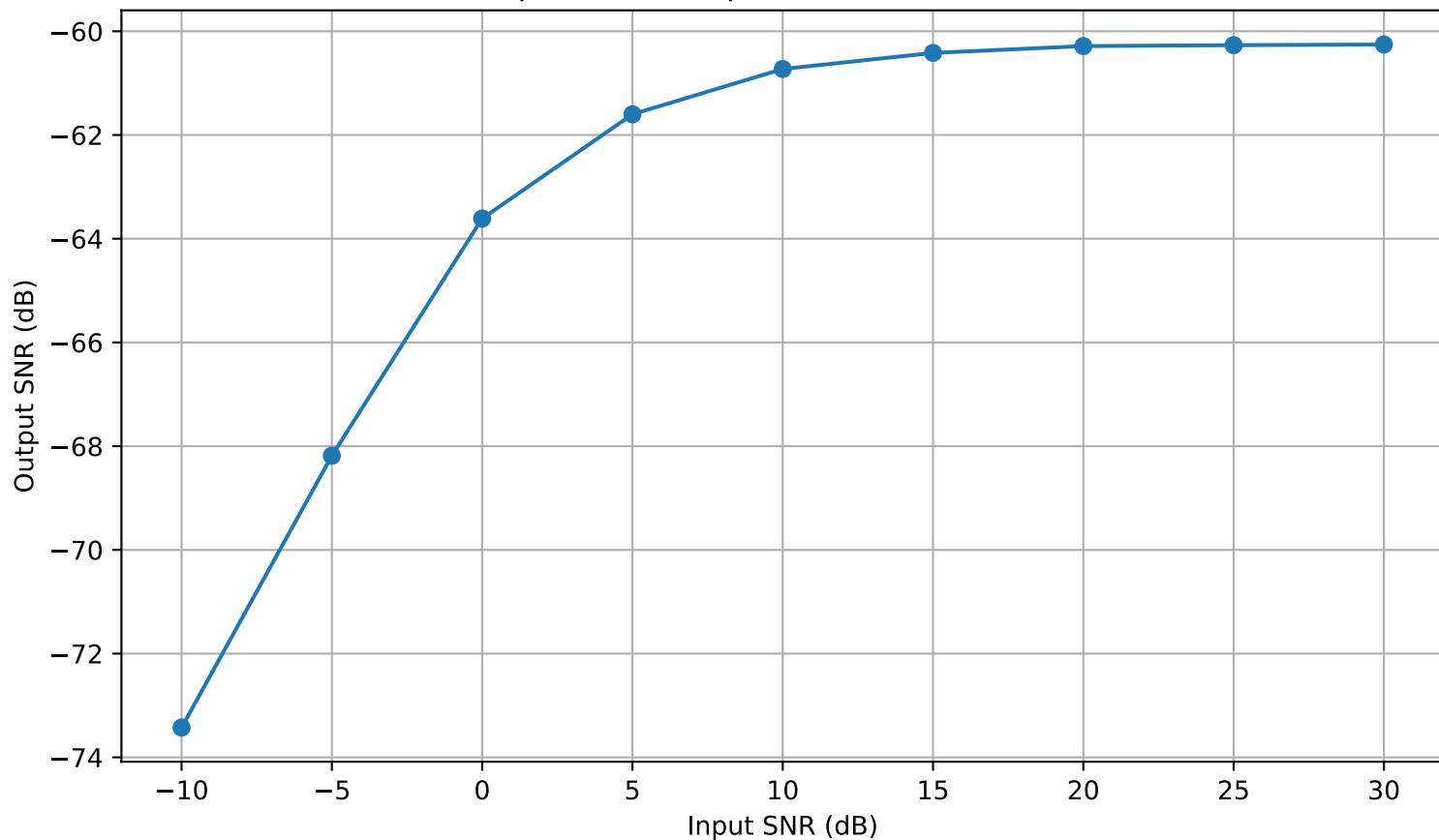
Output SNR vs Input SNR — NBFM SUPER
