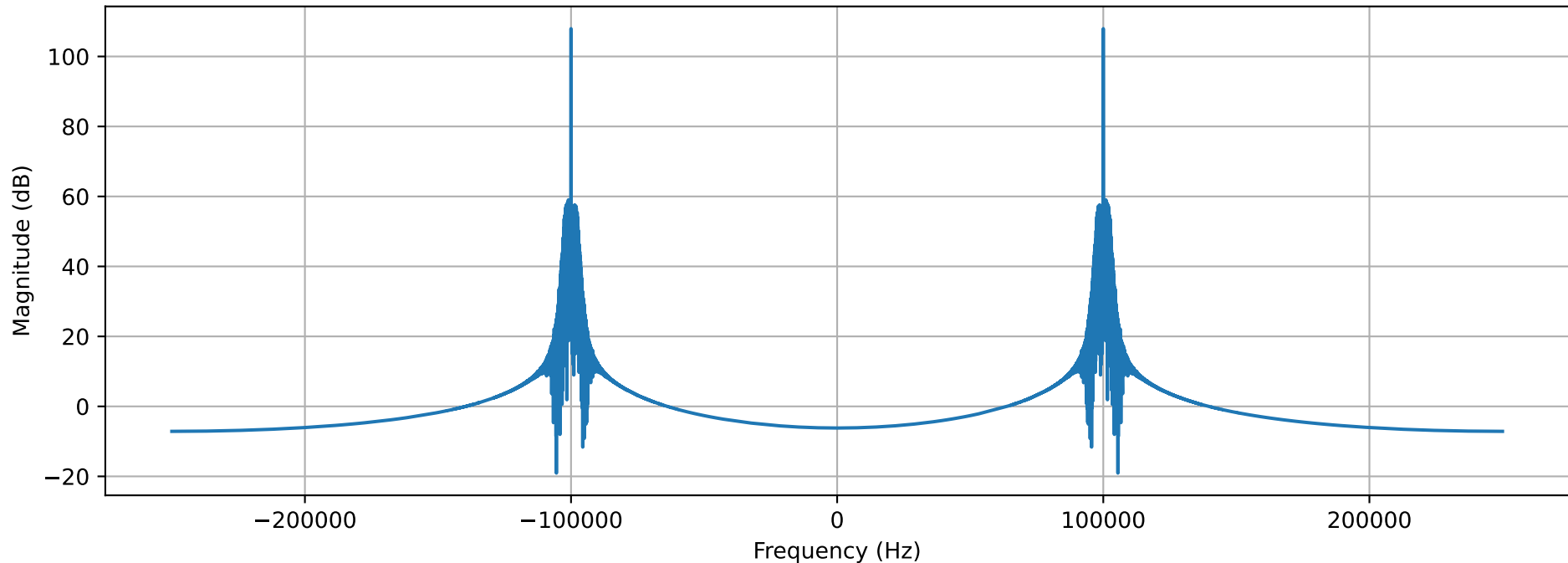
TRF Receiver: RF Bandpass Filter Output
