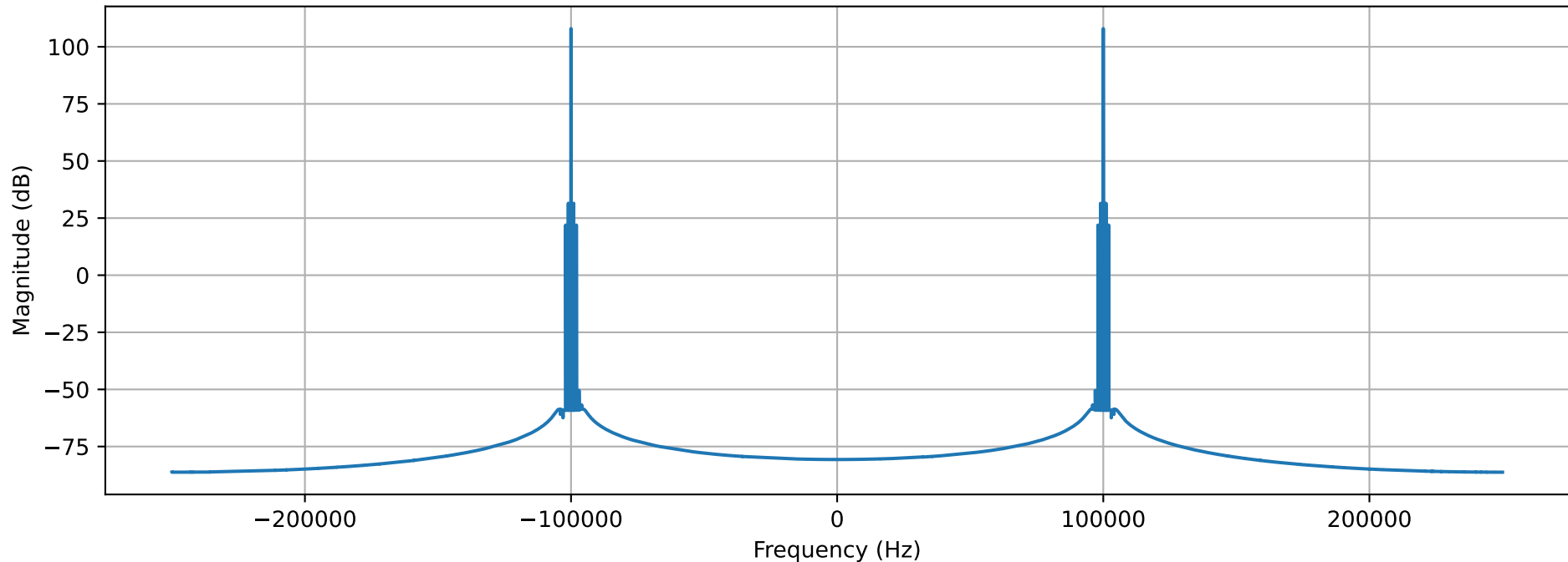
NBFM Spectrum
