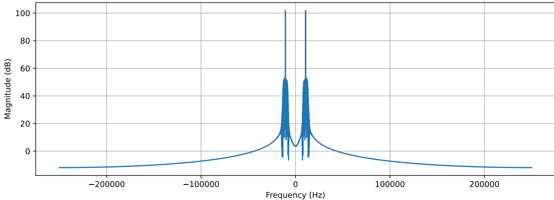
After IF Filter
