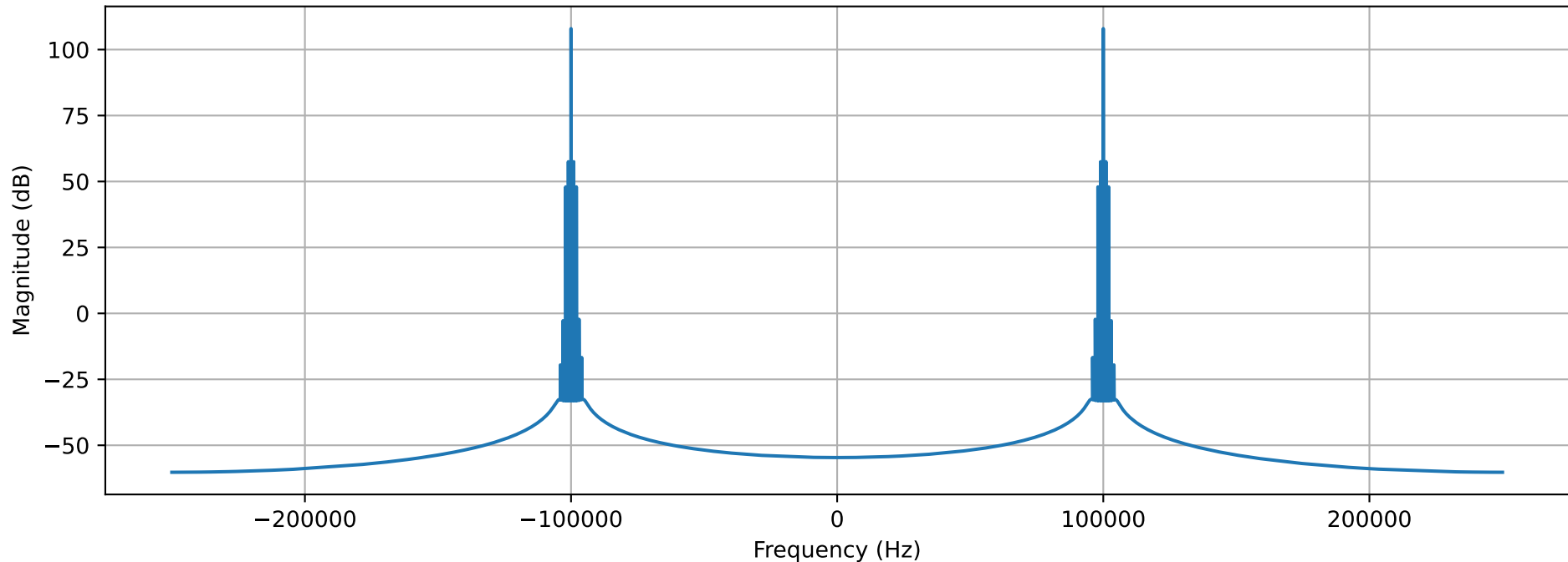
WBFM Spectrum
