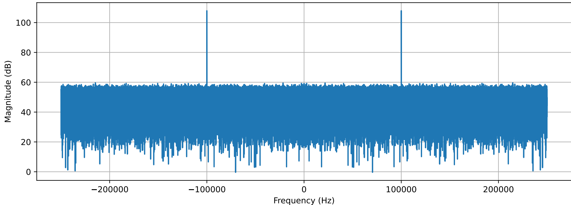
Received RF Signal Spectrum
