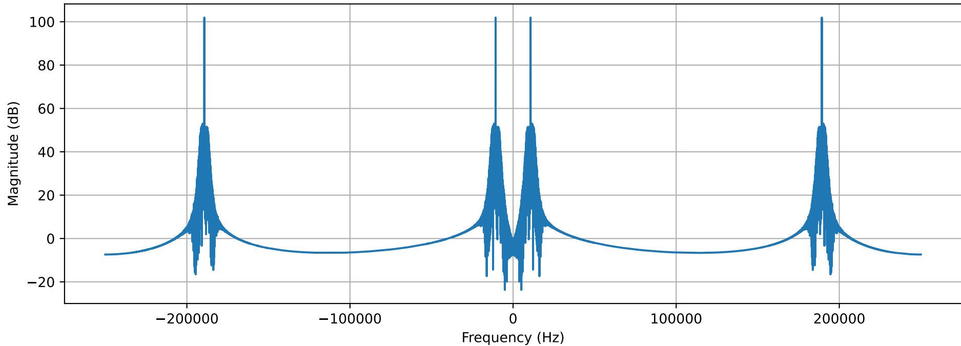
After Mixing (RF \rightarrow IF)
