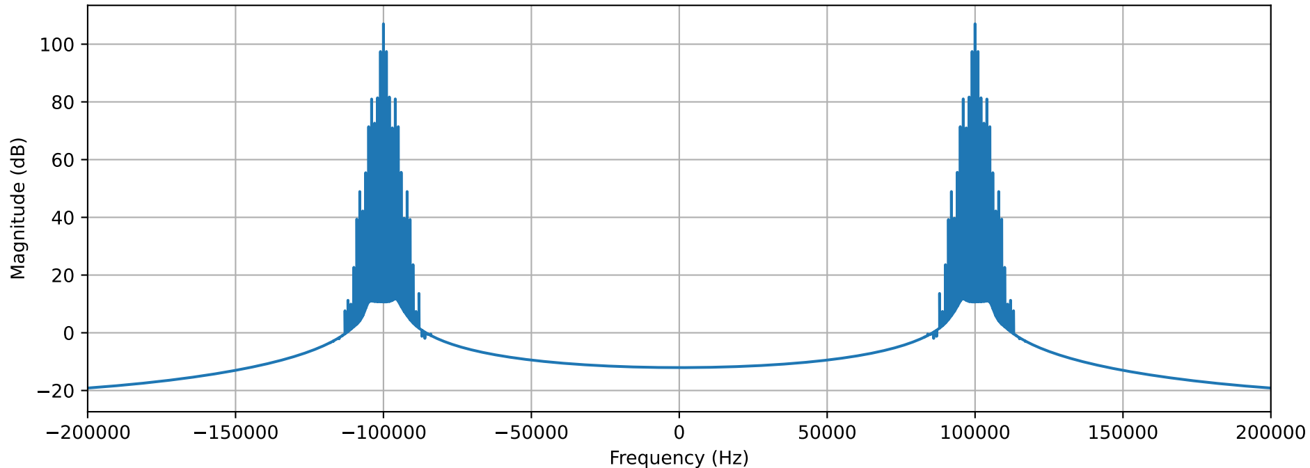
NBFM Spectrum
