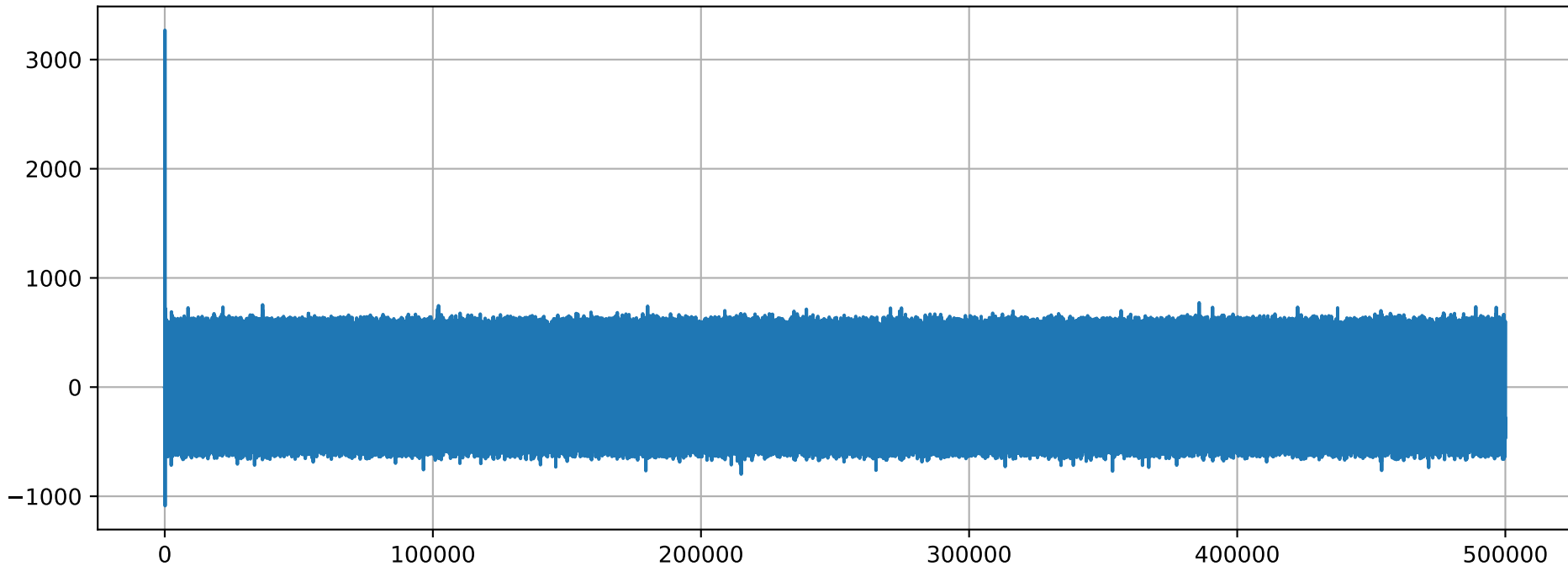
Superhet Receiver Output Audio
