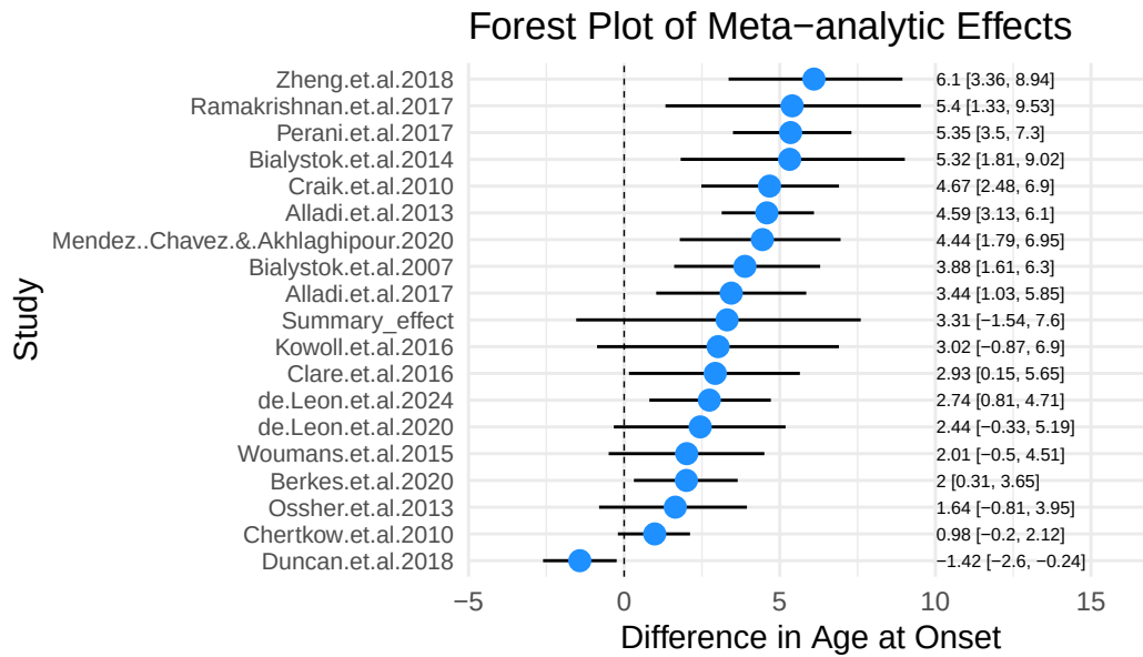
Forest plot of Bilingualism and Age at Onset of Dementia (Note: The estimates and 95% CrI are the differences between bilinguals and monolinguals, so a positive number indicates later onsets for bilinguals.)
