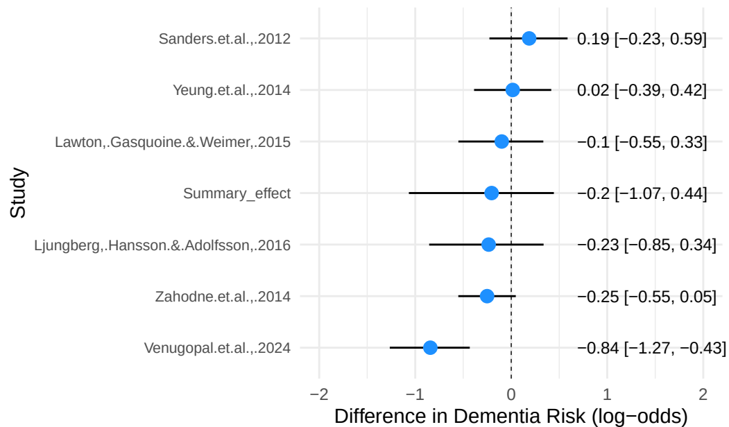
Figure 9. Forest plot of the estimated difference in dementia risk between bilinguals and monolinguals in each study.
