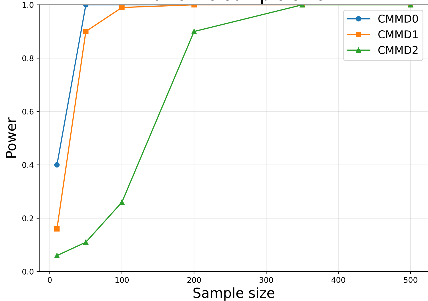
Power vs Sample Size
