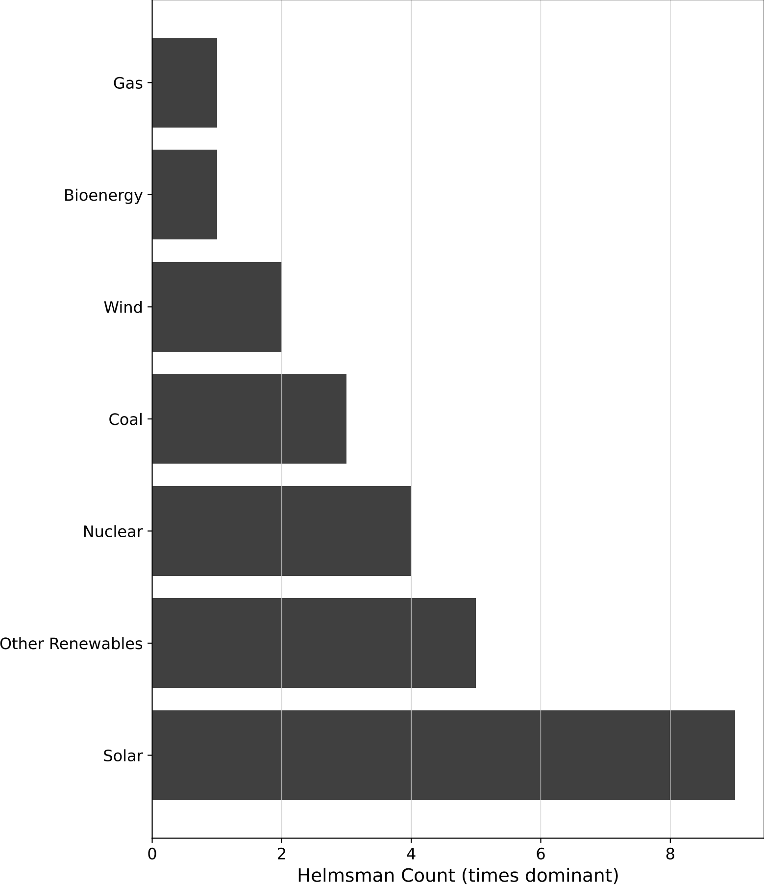
HELMSMAN FREQUENCY
