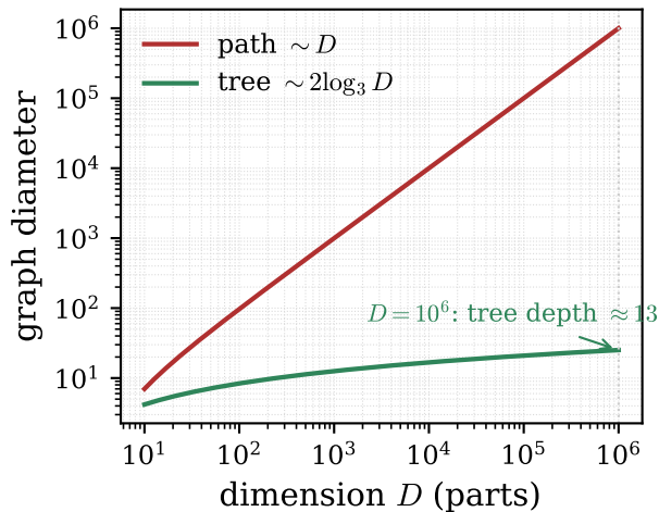
(c) chart-graph diameter
