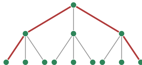
(b) balanced-tree atlas: diameter O(\log D)
