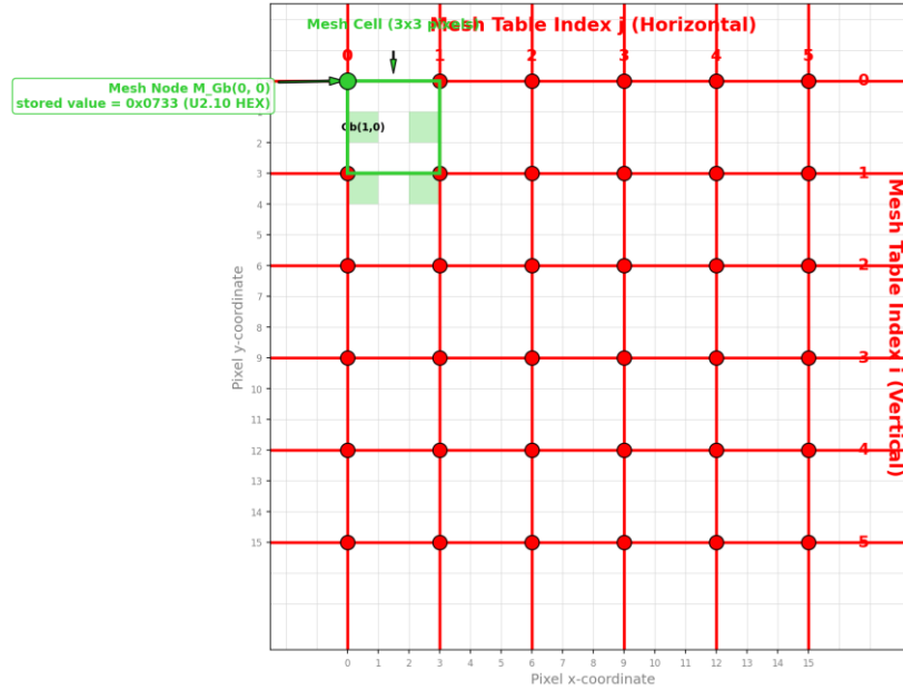
LSC Mesh Grid Mapping Schematic (Example: Gb Channel)
