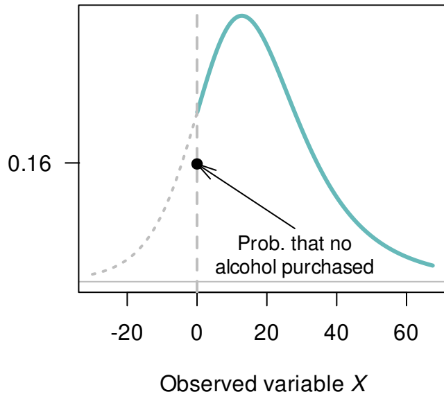
Observed variable X : Average weekly spend on alcohol
