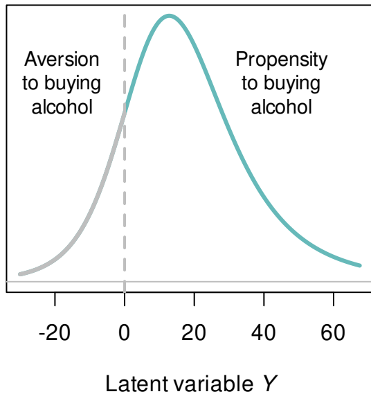
Latent variable Y : Desire to buy alcohol
