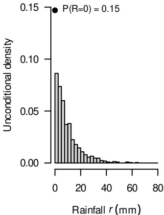
ZM-exponential monthly rainfall
