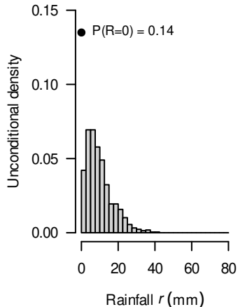
Compound Poisson--gamma monthly rainfall
