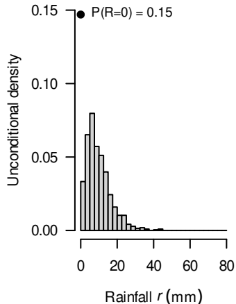
ZM-gamma monthly rainfall
