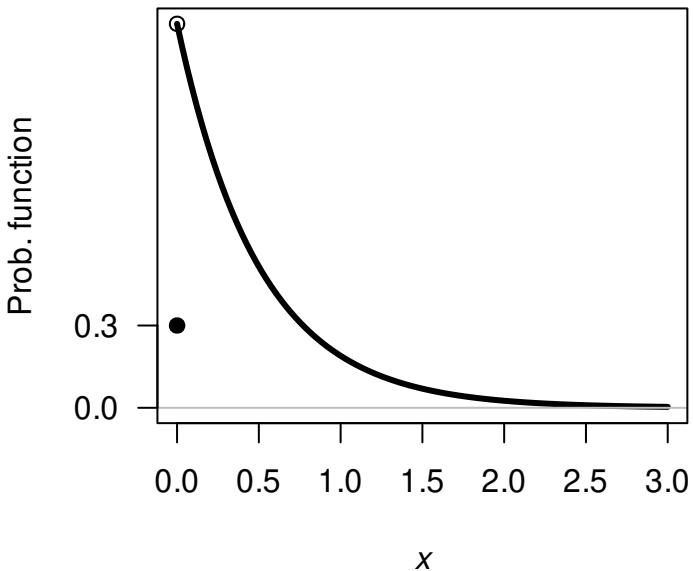
Zero-modified exponential Probability function
