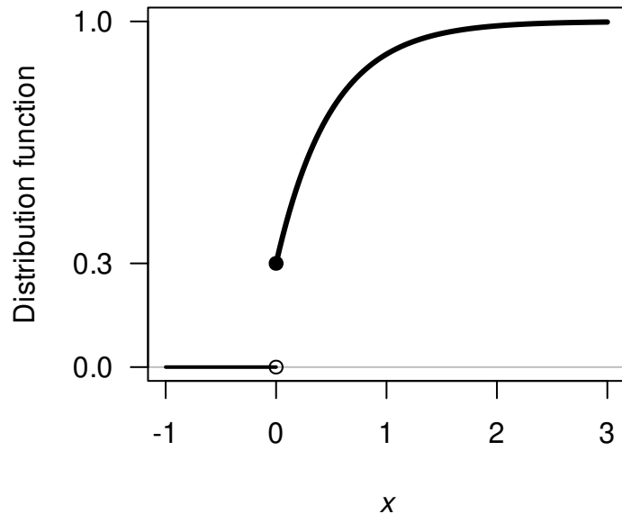
Zero-modified exponential Distribution function
