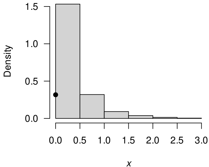
Distribution of X : Mixed random variable
