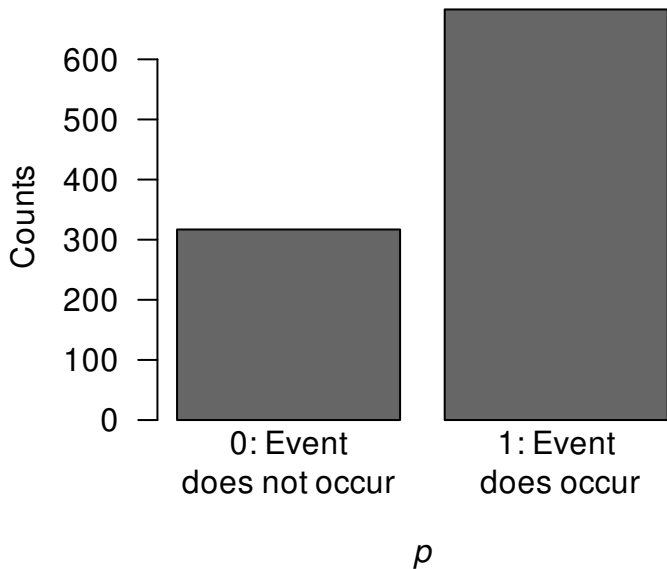
Distribution of p : Prob. of event occurring
