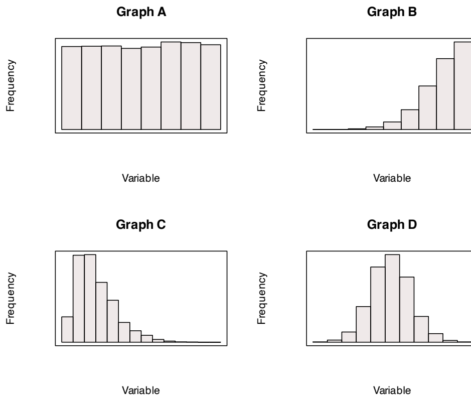
FIGURE 3.2: Four histograms; what shape is appropriate for which scenario?
