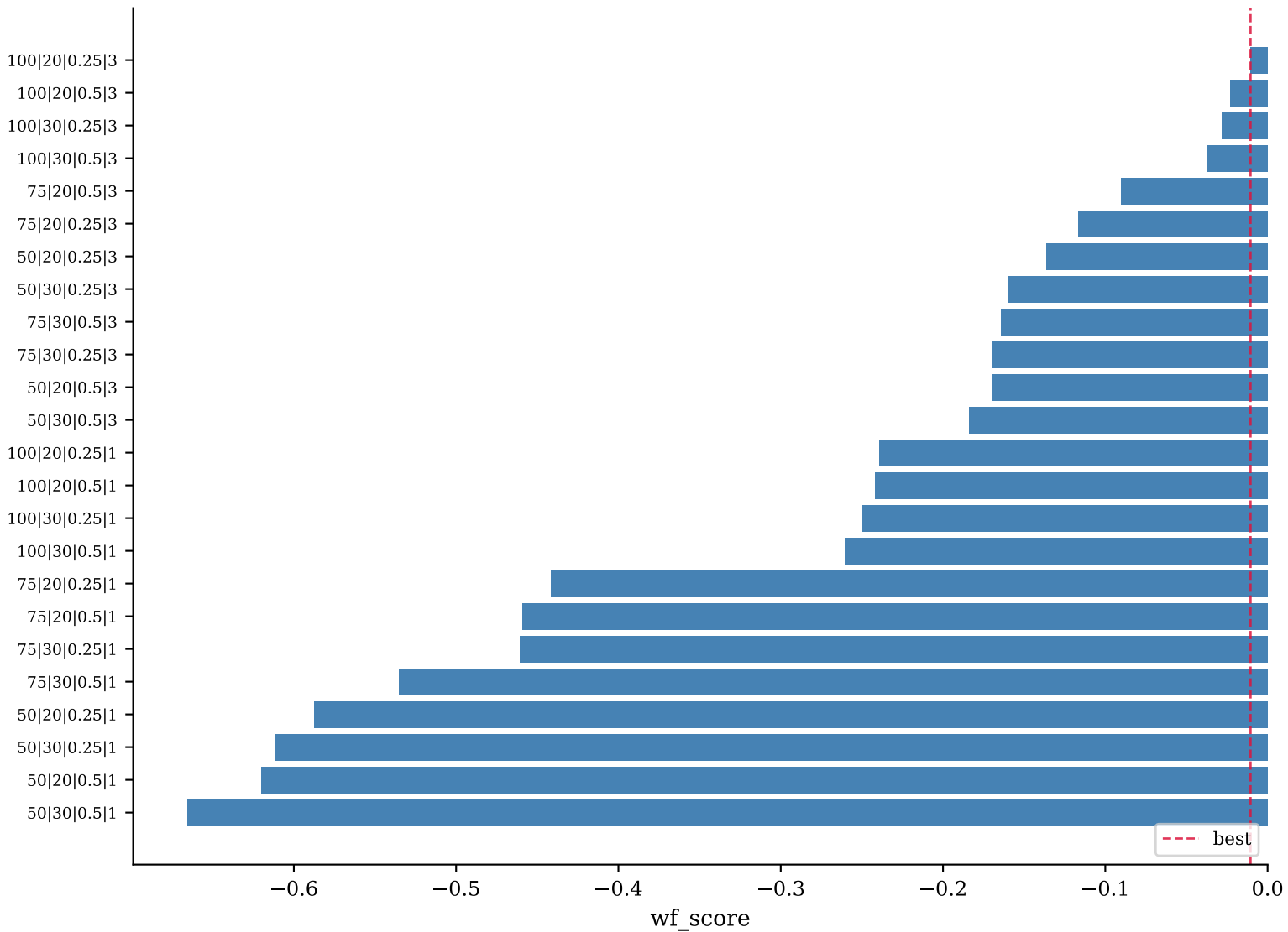
All grid points (MA | VOL | dead-zone | rebalance days)
