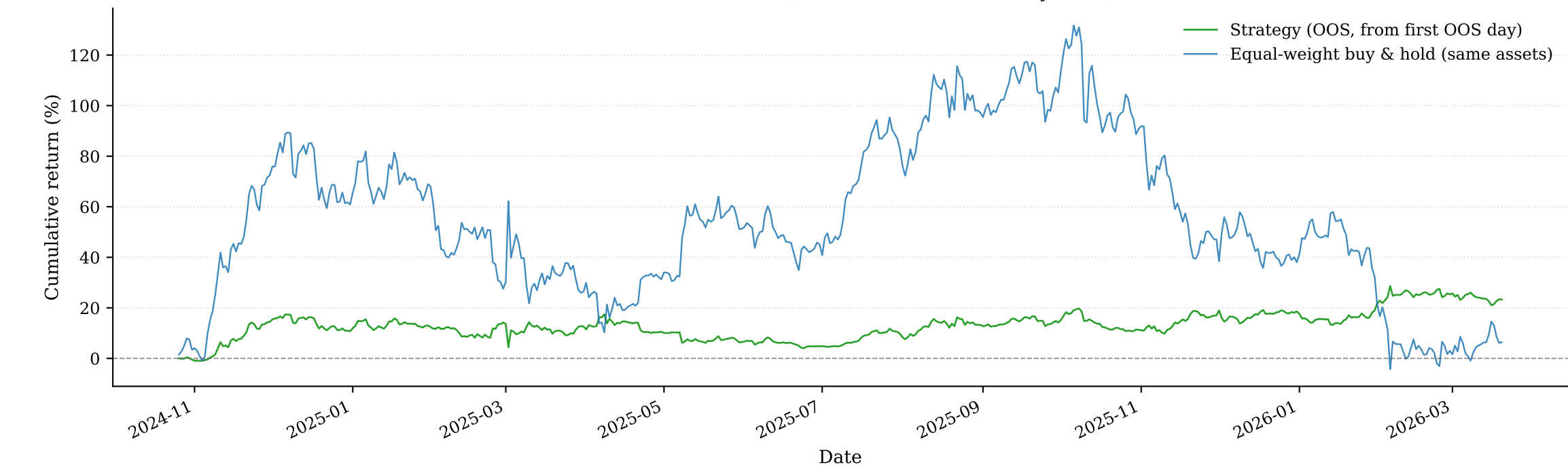
OOS cumulative return (normalized to first OOS day = 0%)
